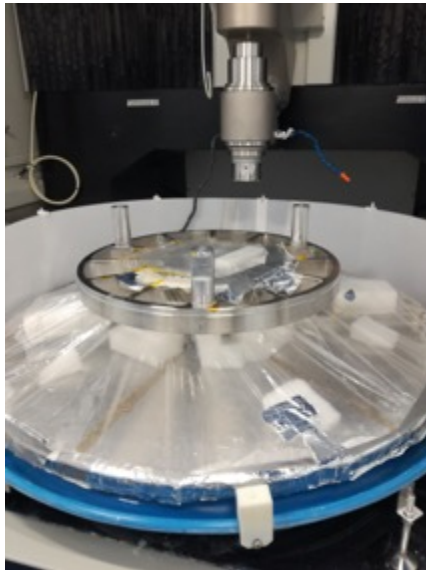
Figure 1: (A) The invar spoke wheel fixed on the Zeeko with new interfaces spacers to allow kinematic repositioning. (B) The system to dismount the shell from the Zeeko.
