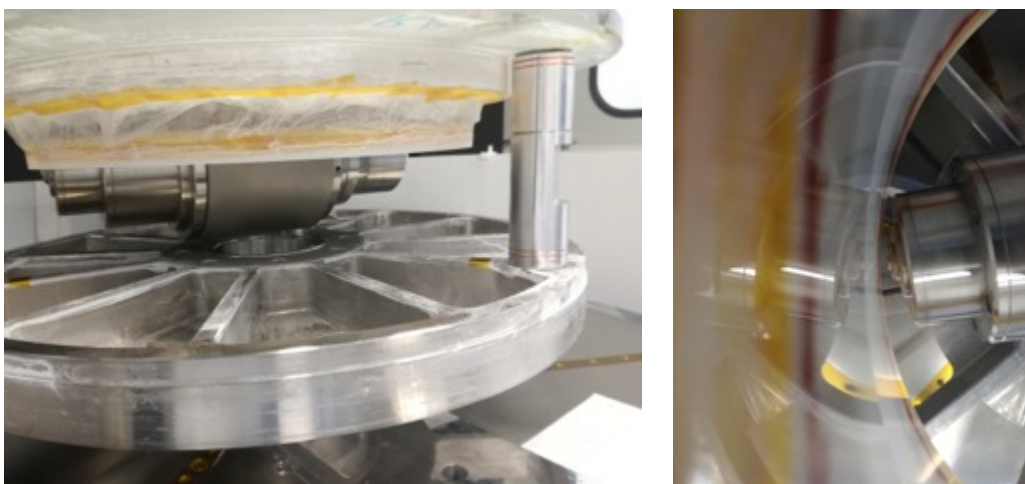
Figure 2: The Zeeko IRP 1200 fit the shell configurations for few millimeters.
