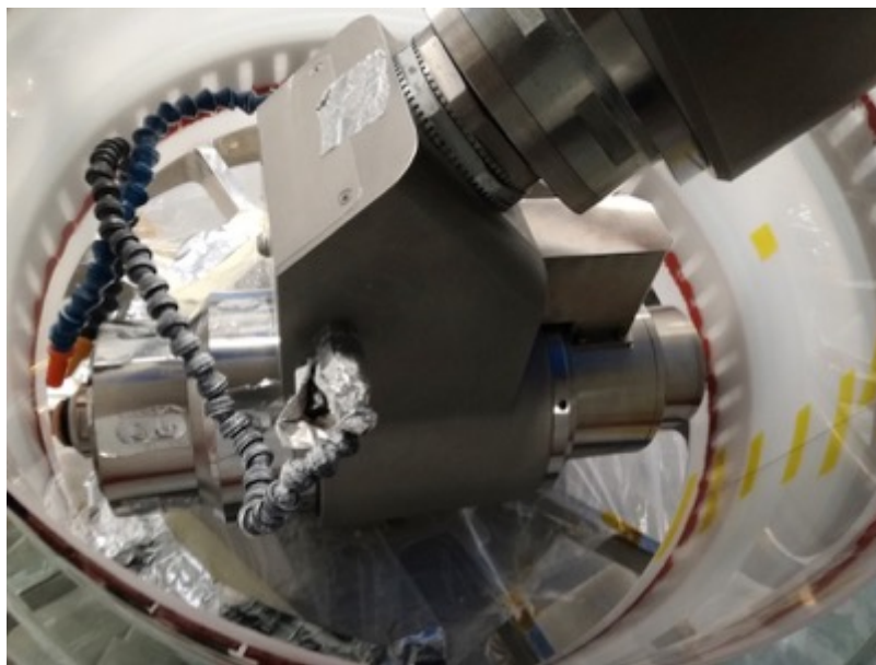
Figure 4: The Zeeko IRP1200 equipped with the Bonnet R20 is used @INAF/OAB to polish an azimuthal segment of the shell#4. Given the relative size of the shell and of the robotic arm, the accommodation of the shell was not simple. The precession angle is reduced to 10° and set in horizontal direction. In this way the shell fits with few millimeters margin. The breakage occurred on the lathe is visible on the right
