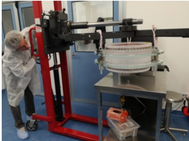
Figure 1: (A) The invar spoke wheel fixed on the Zeeko with new interfaces spacers to allow kinematic repositioning. (B) The system to dismount the shell from the Zeeko.
