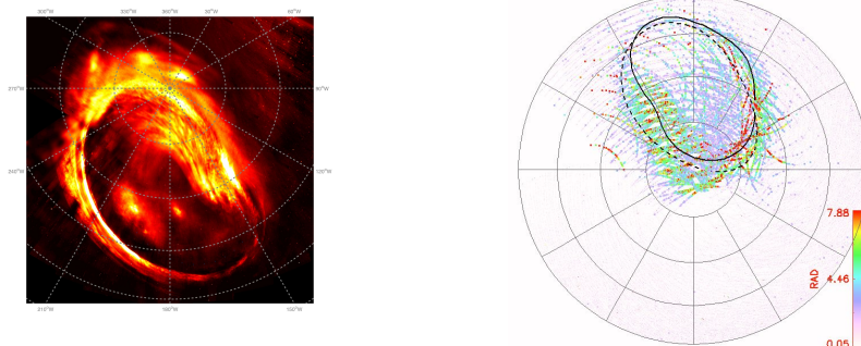
Figure 1. Jupiter north aurora as observed by the imager (left panel), and the spectrometer (right panel)
