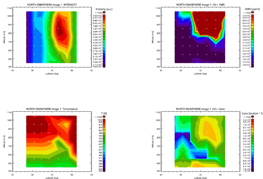
Figure 6. top left panel: integrated intensity of the image 1 spectra, top right panel: retrieved VMR, bottom left panel: retrieved temperature and right bottom panel: concentration of H 3 + (mol/cm 3 ) for image 1. All the maps report the quantities as a function of altitude (y axis) and of the averaged latitude of the limb sequences (x axis).
