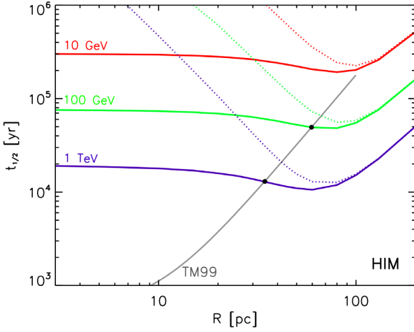
Figure 1. Half-time of the CR cloud (see the text, Section 3) as a function of its initial radius R . The red, green, and purple lines refer to particle energies of 10, 100, and 1000 GeV, respectively. The grey solid line represents the relationship between SNR radius and age according to Truelove & McKee (1999).
