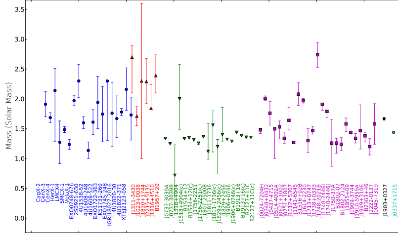
Figure 4: Current NS mass measurements, 68% confidence intervals ( http://jantoniadis.wordpress.com/research/ns-masses/ for original references). Blue - LMXBs; Red - Eclipsing MSPs; Green - DNS; Magenta - NS-WD binaries; Black - MSP-Main Sequence binaries; Cyan - Triple Pulsar. Though some sources may have higher masses than PSRs J1614-2230 and J0348+0432, there are large systematic uncertainties on these measurements or other reasons why they are not as direct or reliable a measurement.
