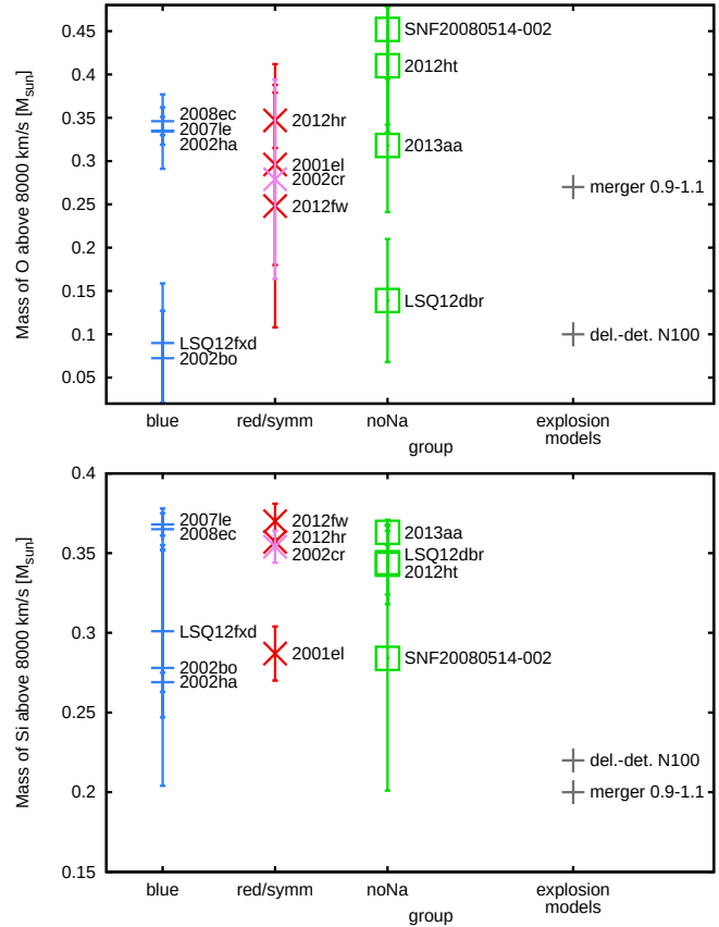
Figure 7. Mass of O ( upper panel ) and Si ( lower panel ) above 8000 \text{ km s}^{-1} in our models, which are grouped according to the narrow Na I D line behaviour of the corresponding SN (left three columns, respectively). The error bars correspond to the error in v_{\text{ph}} ( \pm 1000 \text{ km s}^{-1} , as in Figure 6). For comparison, we plot the corresponding masses within the hydrodynamical explosion/nucleosynthesis models of Röpke et al. (2012) (right column within each panel). The variations in Si mass are actually relatively small (fine mass scale in lower panel) both among our SNe and the hydro models. The merger model ‘compensates’ for its smaller Fe-group mass in the outer layers (Figure 6) by having a larger O abundance and a significant amount of unburned C ( \sim 0.1 M_{\odot} , not plotted).
