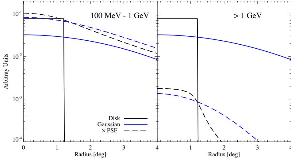
Figure A1. Radial surface brightness profile (arbitrary units) assuming a disk (black-solid line) and a Gaussian emission profile (blue-solid line), folded with the point spread function for P8R2.SOURCE_V6 IRF (dashed lines) for low energies (100 MeV–1 GeV) and at higher energies (>1 GeV). Aside from a different normalization (which however is a free parameter in the likelihood procedure), at low energies, both models cannot be effectively distinguished from one another.
