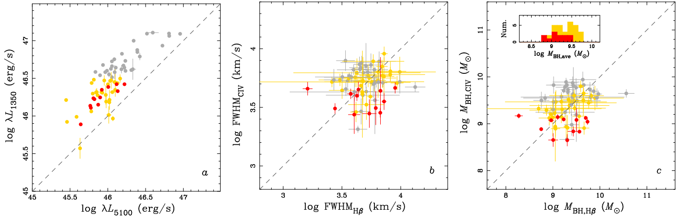
Fig. 6. Comparison of the monochromatic luminosities at 1350 Å and 5100 Å (left, a ), the FWHM of the \text{H}\beta line and the \text{C IV}\lambda 1549 line (middle, b ), and virial black hole masses based on the \text{C IV}\lambda 1549 line and \text{H}\beta line (right, c ). Our sample of N-loud quasars are shown as red circles. Gray and yellow circles denote SDSS normal quasars at 1.5 < z < 2.2 in luminosity ranges of \log \lambda L_{1350} > 46.5 and \log \lambda L_{1350} < 46.5 from Shen & Liu (2012). Errors represent 1\sigma uncertainties of measurements, excluding systematic errors. The one-to-one relations are indicated by dashed lines for each panel.
