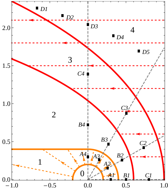
Fig. 2 The geometry of the model: half of the axial section of the system by the plane perpendicular to the line of sight, crossing the pulsar (plane PoS ). The numbers 0 – 4 label the regions with different diffusion modes: 0 is the cold PW, 1 (between the orange curves) is the shocked PW, 2 is the zone near the contact discontinuity, 3 (between the red curves) is the postshock flow of the ISM matter, 4 is the unperturbed ISM. The relative sizes of the regions are not to the scale and depend on the particular properties of a BSPWN. The locations (bins) chosen in the following sections to illustrate simulated particle energy distributions are marked by labelled black squares ( A1 – D5 ). The bins are located at the midpoints of the dashed gray segments of the lines connecting the pulsar and the surfaces, which separate regions 0 – 4 (see §4.2). The gray lines are directed at 0°, 30°, 60°, and 90° with respect to the system symmetry axis.
