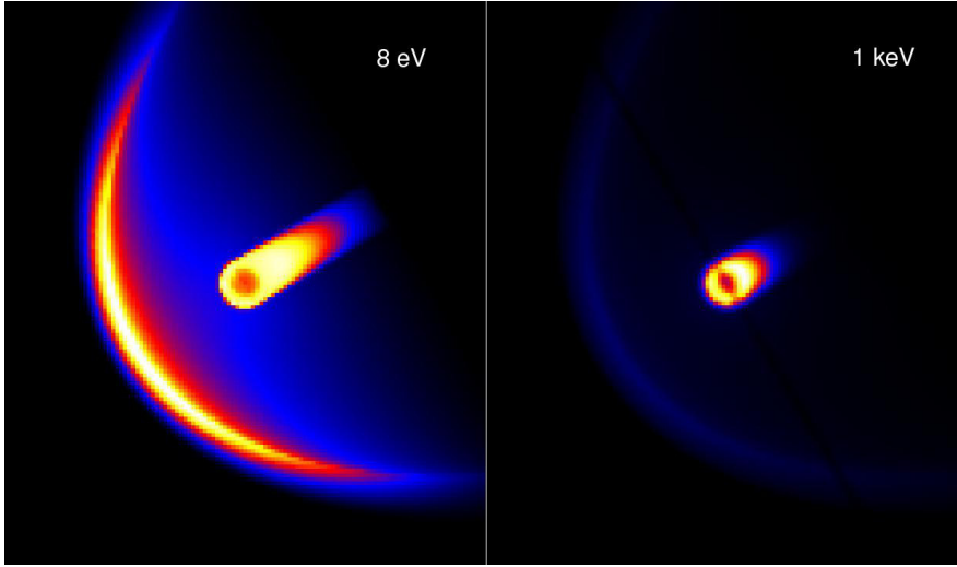
Fig. 4 Simulated synchrotron images of an object similar to J0437-4715, for E = 8 eV ( \approx 1550 Å, left) and 1 keV (right). The absolute intensity is given in normalized units to show the contrast change through the image.
