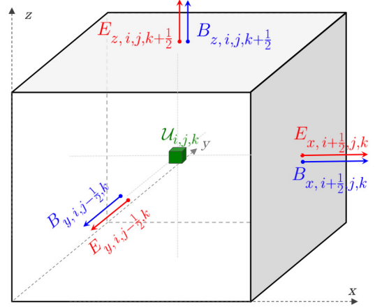
Figure 1. Positioning of hydrodynamical variable ( \mathcal{U}_c in green) and electromagnetic fields ( \mathbf{E}_f and \mathbf{B}_f , red and blue respectively) inside a computational zone (i, j, k) .
