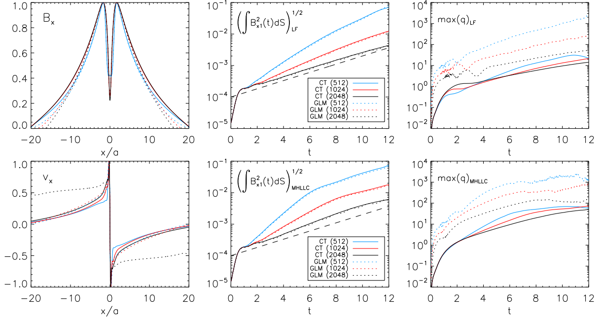
Figure 9. Left panels: profiles of the x-components of magnetic field (top) and velocity (bottom) for the tearing mode instability at t = 10 using different methods and resolutions. The 1D cuts are taken along the x-axis for y = 0 and y = 3/4L_y , respectively and are normalized to unity. Solid (dotted) lines corresponds to the solutions obtained with the CT (GLM) methods while colors denote the different grid resolutions used N_x \times N_x/4 (green, red and black stand for N_x = 512, 1024, 2048 , respectively). Middle panels: measured growth rates for the selected cases using the LF solver (top) and the MHLHC solver (bottom). Right panels: maximum value of the charge as a function of time.
