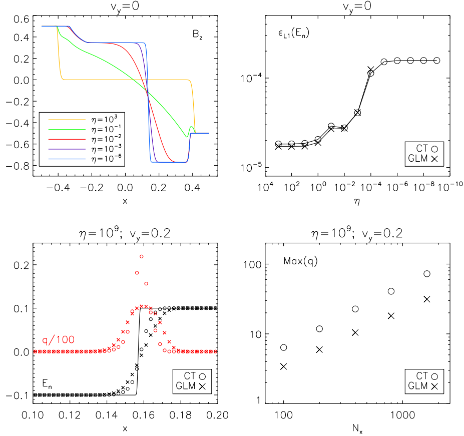
Figure 5. Results for the 2D rotated shock tube problem at t = 1/\sqrt{1+\tan^2\alpha} . The y component of the magnetic field (in the original unrotated frame) is plotted in the top-left panel for selected values of the \eta as reported in the legend. In the top-right panel we plot the L1-norm errors of the normal component of electric field for the GLM and CT schemes as a function of \eta . In the bottom panels we show the normal component of \mathbf{E} as well as the charge (red symbols, divided by 100) for the second variant of the problem (left) and the maximum value of the charge as a function of the grid resolution (right). Results obtained with the CT and GLM schemes are shown using circles and crosses.
