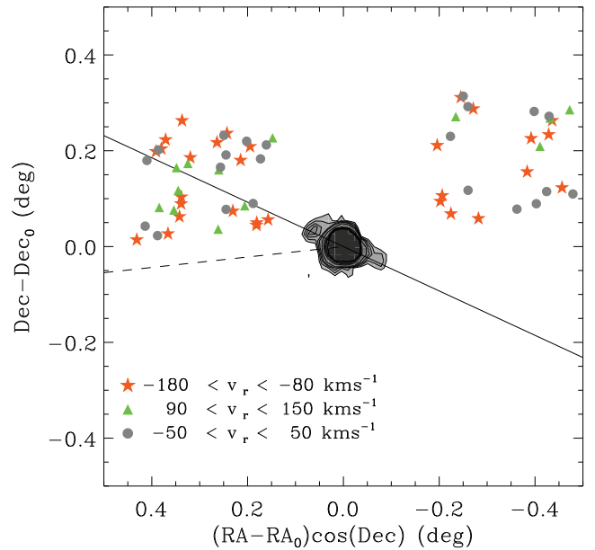
Figure 4. Density map generated for an area of 1 \times 1 \text{ deg}^2 centred in the coordinates of Whiting 1 [RA_0, Dec_0] = [30^\circ 73', -03^\circ 25'] . Isodensity lines are drawn at levels of 3, 3.5, 4, 5, 7.5, 9, 10 and >12 times the mean background level. The solid line indicates the mean orbit of the Sgr tidal stream along that line of sight according to PR10, whereas the dashed line indicates the direction of the Milky Way centre. The symbols indicating the position of target stars are colour-coded according to the velocity ranges indicated in the legend.
