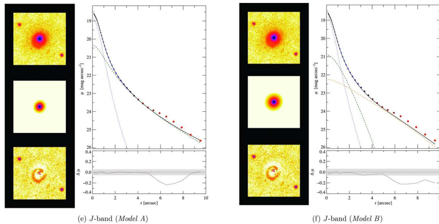
Figure 10. Two-dimensional surface-brightness profile decomposition of 1H 0323+342 in J -band for Model A (PSF+Bulge; left panel) and Model B (PSF+Bulge+Disc; right panel). Top left subpanel: the observed image in a field of view of 20 arcsec \times 20 arcsec. Middle left subpanel: model used to describe the surface brightness distribution. Bottom left subpanel: the residual image. Top right subpanel: radial profile of the surface brightness distribution. The filled circles show the observations, and the solid, pointed, and dashed lines represent the model, PSF, and host galaxy, respectively. The exponential disk component is shown in orange. Bottom right subpanel: residuals. Adapted from [181].
