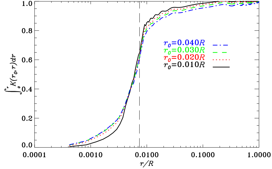
Figure 7. OLA cumulative integrals of the averaging kernels centered at different locations in the H-burning shell. The dashed black line indicates the location of the inner edge of the H-burning shell.
