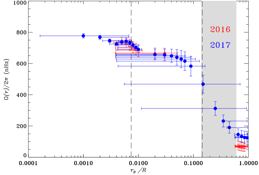
Figure 5. Internal rotation of KIC 4448777 at different depths as obtained by the OLA inversion with data of Paper I (flagged by 2016 in red ) and present data (flagged by 2017 in blue). Vertical error bars are 2\sigma of the standard deviations. The dashed lines indicate the base and the external edge of the H-burning shell. The shaded area marks the region inside the star where the spatial resolution becomes low.
