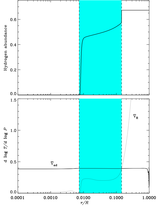
Figure 3. Hydrogen content (upper panel) and temperature gradients (lower panel) in Model 2 of KIC 4448777. The extent of the core and the base of the convective envelope located respectively at r_{He} = 0.0074R and r_{cz} = 0.1448R are shown by the dashed lines. In the lower panel the solid line shows the adiabatic gradient \nabla_{ad} and the dotted line shows the radiative gradient \nabla_R . The H-burning shell is shaded in light blue.
