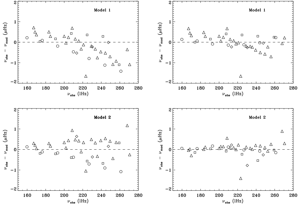
Figure 2. Differences between modelled and observed frequencies plotted against observed frequencies for Model 1 (upper row) and Model 2 (lower row) without correction (panels on the left) and with surface corrections (panels on the right). Circles are used for modes with l = 0 , triangles for l = 1 , squares for l = 2 , diamonds for l = 3 .
