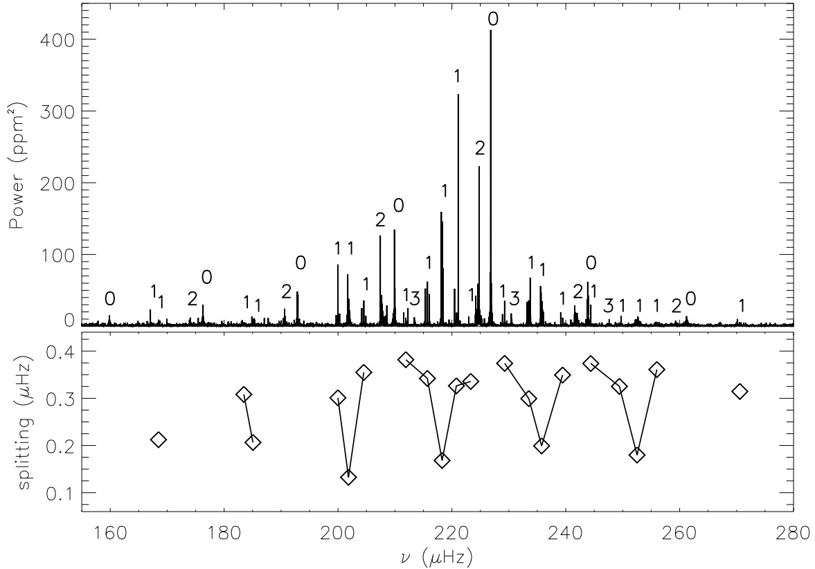
Figure 1. Panel a: Observed frequency spectrum of KIC 4448777. The harmonic degrees of the modes ( l = 0, 1, 2, 3 ) are indicated. Multiplets due to rotation are visible for l = 1 . Panel b: Observed rotational splittings for l = 1 modes.
