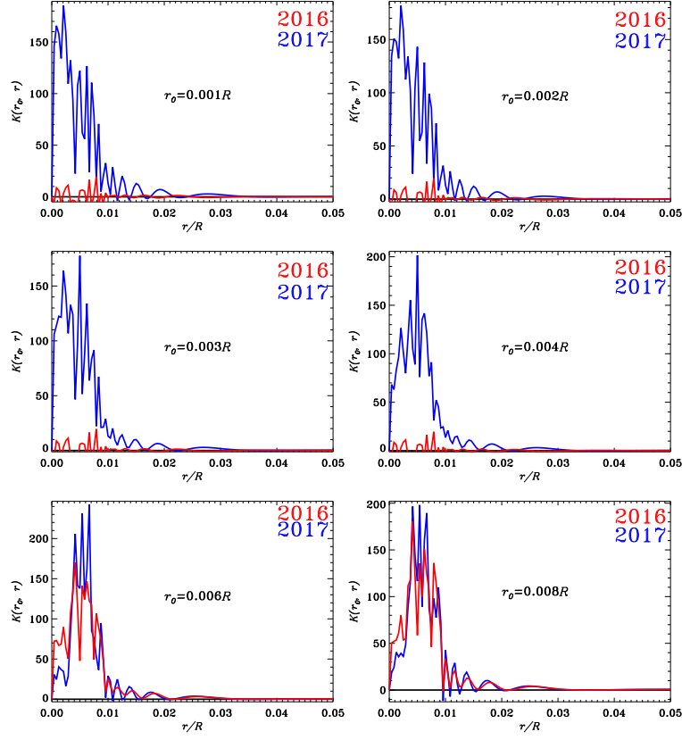
Figure 6. Averaging kernels for OLA inversion indicating localization of the solutions inside the He core and part of the H-burning shell as obtained by using present data (blue line) and data of Paper I (red line).
