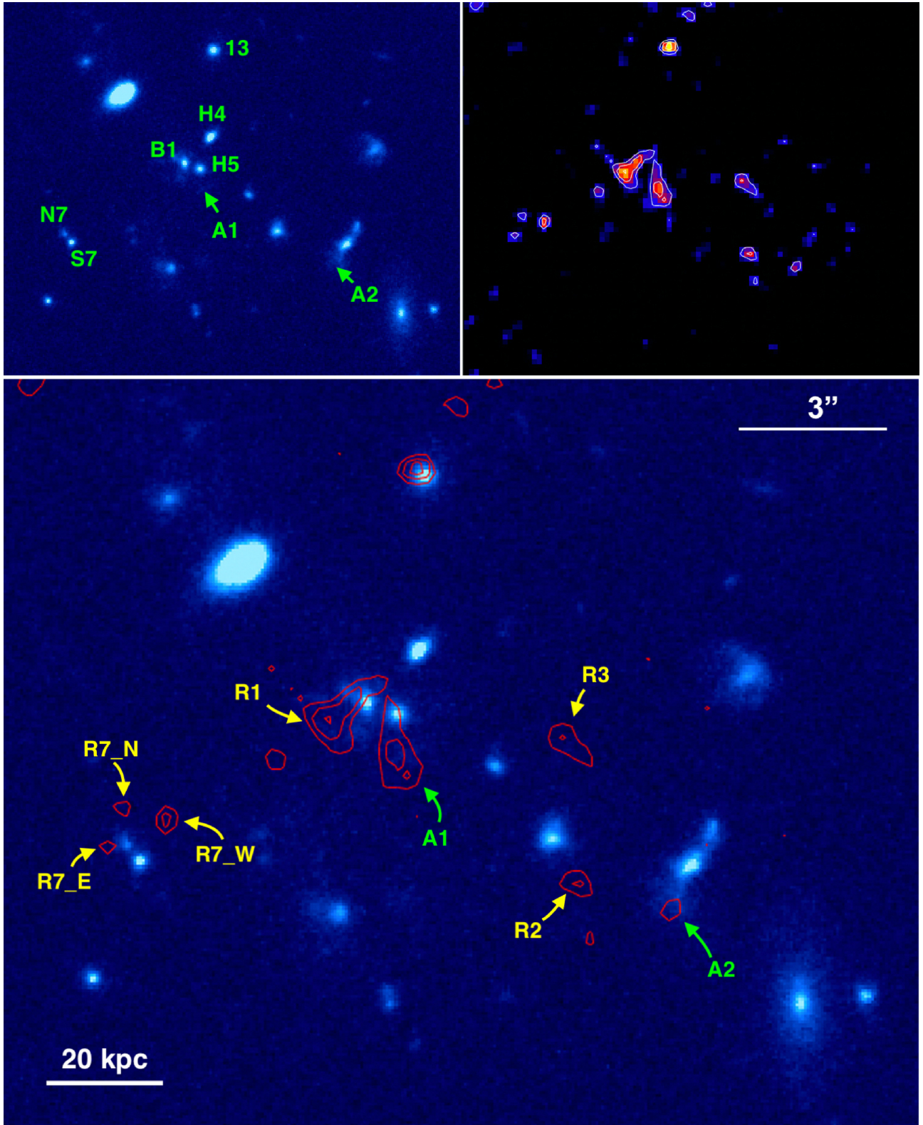
Figure 5. Top left: The HST /WFC3 F140W image with the sources listed in Table 1 marked. However, 2 and A6 are not shown as they are outside the area shown and are not relevant to the results presented in this work. Top right: The 3 GHz VLA image of the region with sigma contours starting at 3\sigma with 1\sigma increments, as in Fig. 3. Bottom: The same HST /WFC3 F140W image with the contours of the VLA 3 GHz image along with the AGN jets listed in Table 2 (in yellow) and the two HST undetected bright ALMA sources A1 and A2 that are also detected at 3 GHz (in green) marked.
