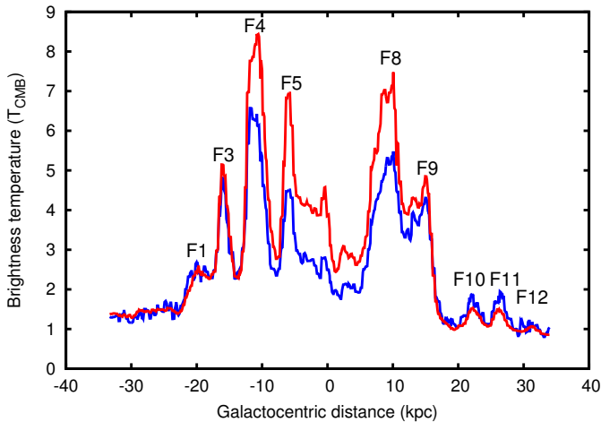
Fig. 4. Cut along the major axis of M31. Negative values are on the higher declination side of the galaxy. The red line is 857 GHz (350 \mu\text{m} ) and the blue line is 353 GHz (850 \mu\text{m} ) rescaled by a factor of 1000. Various spiral arm structures, including the outermost rings at 20–30 kpc, are clearly visible at both frequencies. Fields are numbered as per Fig. 3.
