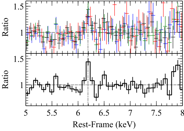
Figure 8. The ratio of the residuals to a continuum fit of the form \text{TBABS} \times (\text{PL} + \text{PL}) to the long-term 2014/2013 EPIC-pn difference spectra from 5 to 8 keV. The upper panel shows the four individual observations: 2014a (black), 2014b (red), 2014c (green) and 2014d (blue). Meanwhile, for extra clarity, the lower panel shows the residuals of the difference spectrum where the 2014 data have been combined into a single spectrum. A clear excess of emission remains at \sim 6.2 keV.
