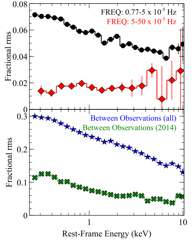
Figure 10. The 0.3–10 keV EPIC-pn rms spectra of Ark 120. Upper panel: the within-observation rms spectra, averaged over all observations acquired in 2014. The circles (black) and diamonds (red) correspond to a lower 0.77\text{--}5 \times 10^{-5} and a higher 5\text{--}50 \times 10^{-5} Hz frequency range, respectively. Lower panel: the long-term ‘between-observation’ rms spectra averaged over the four 2014 orbits (green crosses) and all observations (blue stars), respectively. See Section 3.1.2 for details.
