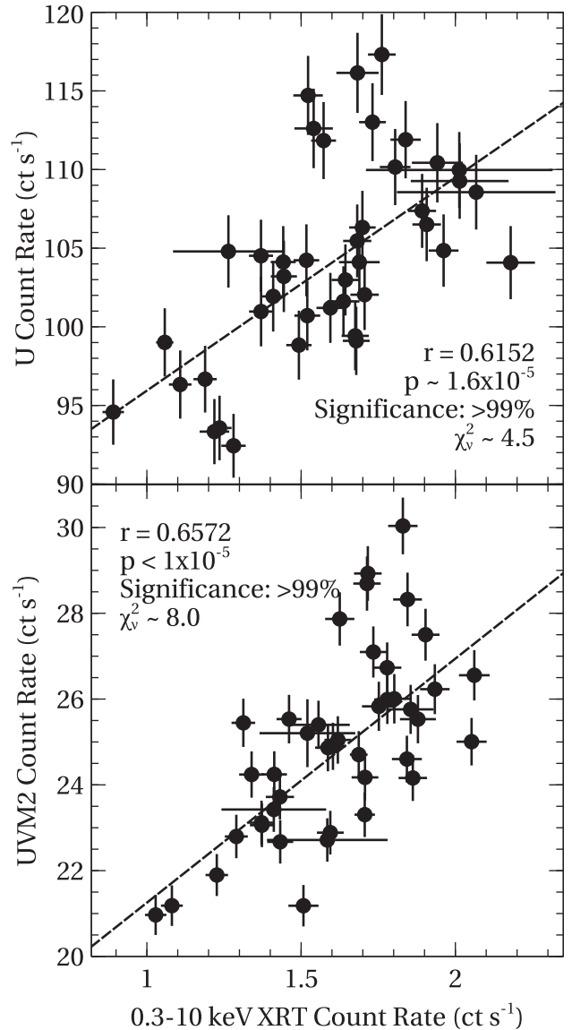
Figure 18. The 0.3\text{--}10 keV XRT count rate plotted against the U (upper panel) and UVM2 (lower panel) bands. In each case, a function of the form U = aX + b is fitted to the data, indicating a clear positive trend. The reduced \chi^2 values are included on the plot.
