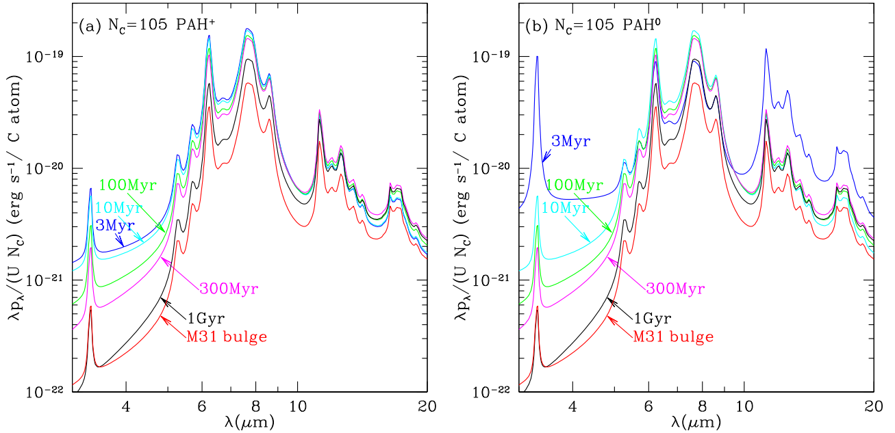
Figure 7. Emission per C atom for N_C = 105 \text{PAH}^0 and \text{PAH}^+ when heated by radiation with the spectrum of the M31 bulge, and single-age Z = 0.02 stellar population models from BC03.
