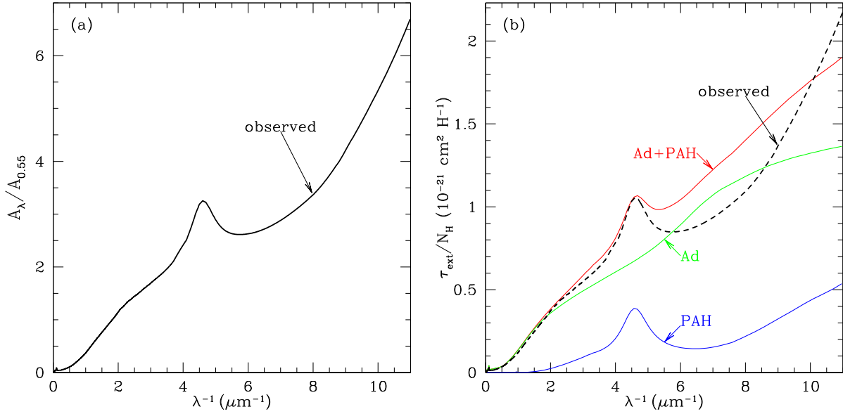
Figure 2. (a) Dust extinction in the diffuse ISM used in Equation (7) (from Hensley & Draine 2021). (b) Extinction calculated for adopted size distributions of astrodrust (Ad) and PAH (Equations (14) and (15)). The broken curve is observed extinction (see panel (a)).
