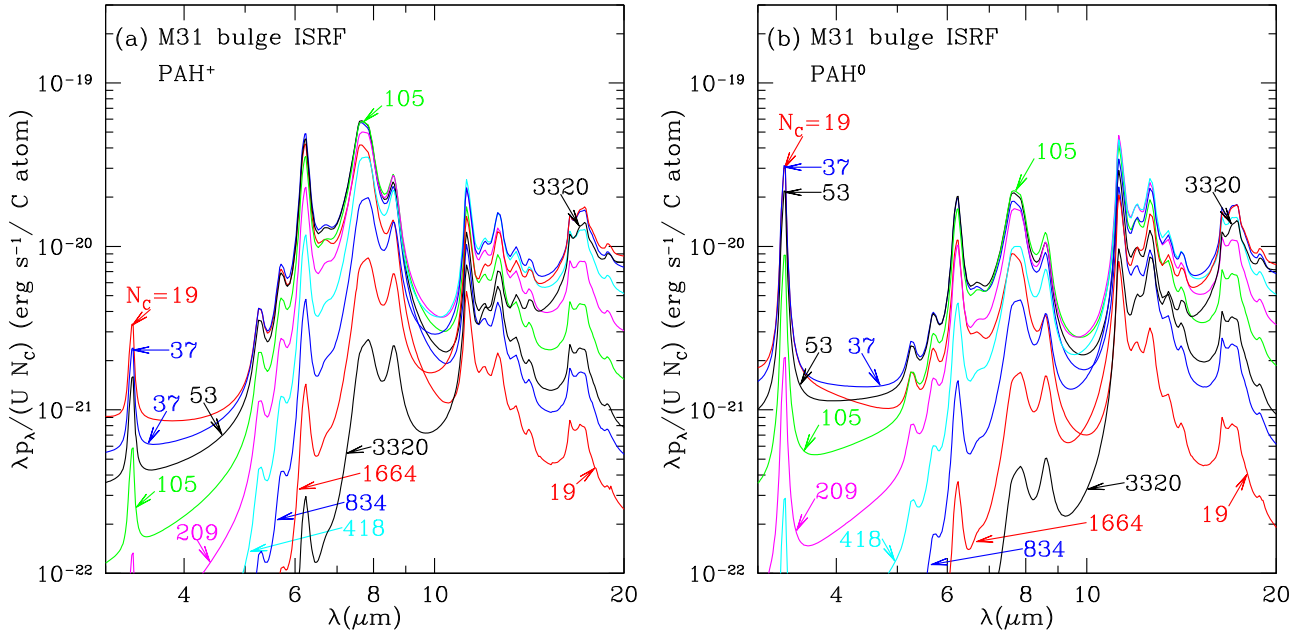
Figure 5. Same as Figure 4, but for heating by starlight from the M31 bulge population.
