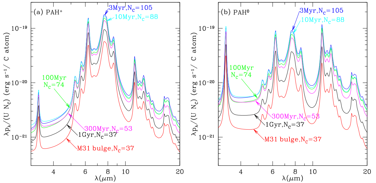
Figure 8. Emission per C atom for \text{PAH}^0 and \text{PAH}^+ when heated by various radiation fields, for sizes giving \langle h\nu \rangle_{\text{abs}}^{(\text{PAH})} = 0.08 \text{ eV} ( \langle h\nu \rangle_{\text{abs}}/N_C \approx 0.08 \text{ eV} , where \langle h\nu \rangle_{\text{abs}} is the mean absorbed photon energy (see the text). The single-age stellar population spectra are from BC03. Except for the reddest spectra (M31 bulge and 1 Gyr old starburst), the PAH emission spectra are very similar provided \langle h\nu \rangle_{\text{abs}}^{(\text{PAH})}/N_C \approx \text{const.}
