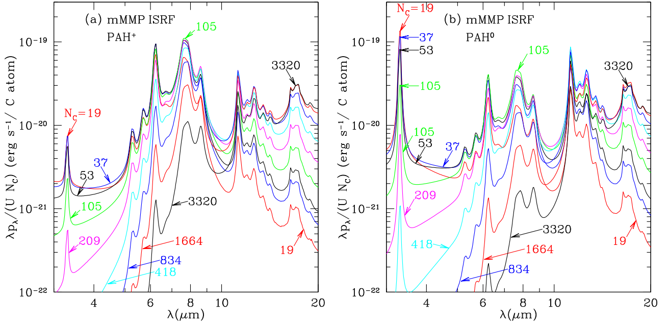
Figure 4. Emission per C atom for (a) PAH ions and (b) neutrals of various sizes, when heated by the mMMP ISRF. The spectra shown are calculated for U = 1 , but p_\lambda/U is nearly independent of U for \lambda < 20 \mu\text{m} and U \lesssim 10^2 .
