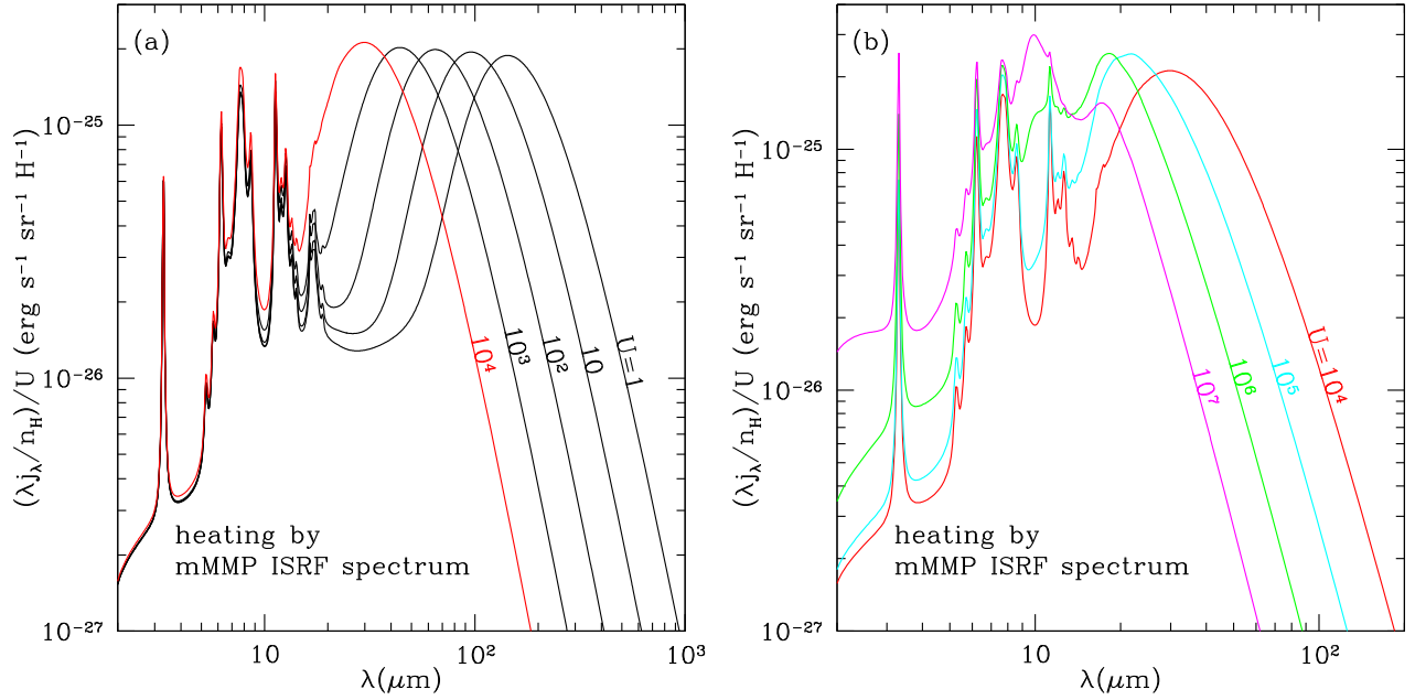
Figure 10. Emission spectra for standard dust mixture heated by radiation with mMMP ISRF spectrum and varying U , for standard PAH size distribution ( a_{01} = 4 \text{ \AA} ) and standard \text{PAH}^+ fraction f_{\text{ion}} (see the text). (a) U \leq 10^4 ; (b) U \geq 10^4 .
