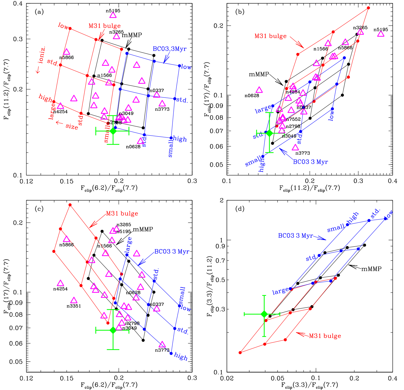
Figure 21. Selected model PAH band ratios calculated for three different starlight spectra (3 Myr old starburst, mMMP radiation field, and M31 bulge spectrum). Band ratios shown are for U = 1 , but apply for U \lesssim 10^3 . Results (dots) are shown for three size distributions (“small,” “std,” and “large”), and three ionization models (“low,” “std,” and “high”). Triangles show measured ratios for 25 SINGS galaxies (see the text). The green diamond shows band ratios for the 1C galaxy sample of Lai et al. (2020), with error bars showing the first through ninth decile range within the 1C sample.
