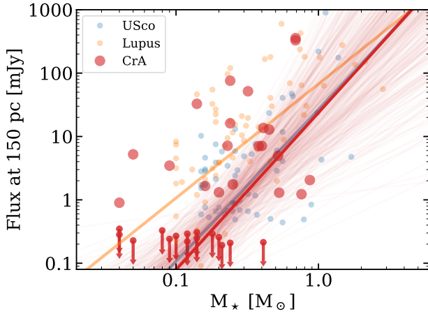
Fig. 5. Correlation between dust disk flux scaled at 330 GHz (assuming \alpha = 2.25 , as in Ansdell et al. 2018) and at a distance of 150 pc with stellar mass for the objects in CrA. The slopes of Lupus and Upper Sco are also plotted for comparison. We show the results of the Bayesian fitting procedure by Kelly (2007). The solid line represents the best-fit model, while the light lines show a subsample of models from the chains, giving an idea of the uncertainties.
