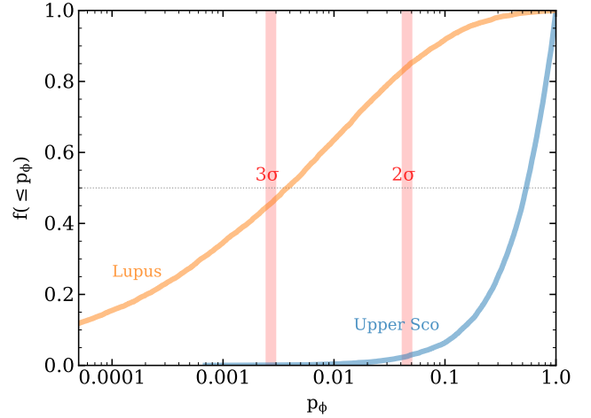
Fig. 7. Comparison of the mass distributions of Lupus and USco to that of CrA, following the MC analysis proposed by Andrews et al. (2013) . p_\phi is the probability that the synthetic population drawn from the comparison sample (Lupus and Upper Sco) and the reference sample come from the same parent population. f(< p_\phi) is the cumulative distribution for p_\phi resulting from the logrank two-sample test for censored datasets after 10^4 MC iterations.
