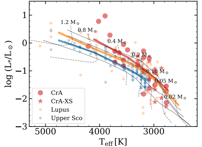
Fig. 6. HR diagram showing the sources in our CrA sample (red), in the Lupus sample from Ansdell et al. (2016) (orange), and in the Upper Sco sample (blue) from Barenfeld et al. (2016). The evolutionary tracks for different stellar masses and the relative isochrones from Baraffe et al. (2015) are also plotted for reference. The isochrones refer (from top to bottom) to the 1, 2, 5, and 10 Myr isochrones. The colored solid lines show the approximate median value of the luminosity at each temperature.
