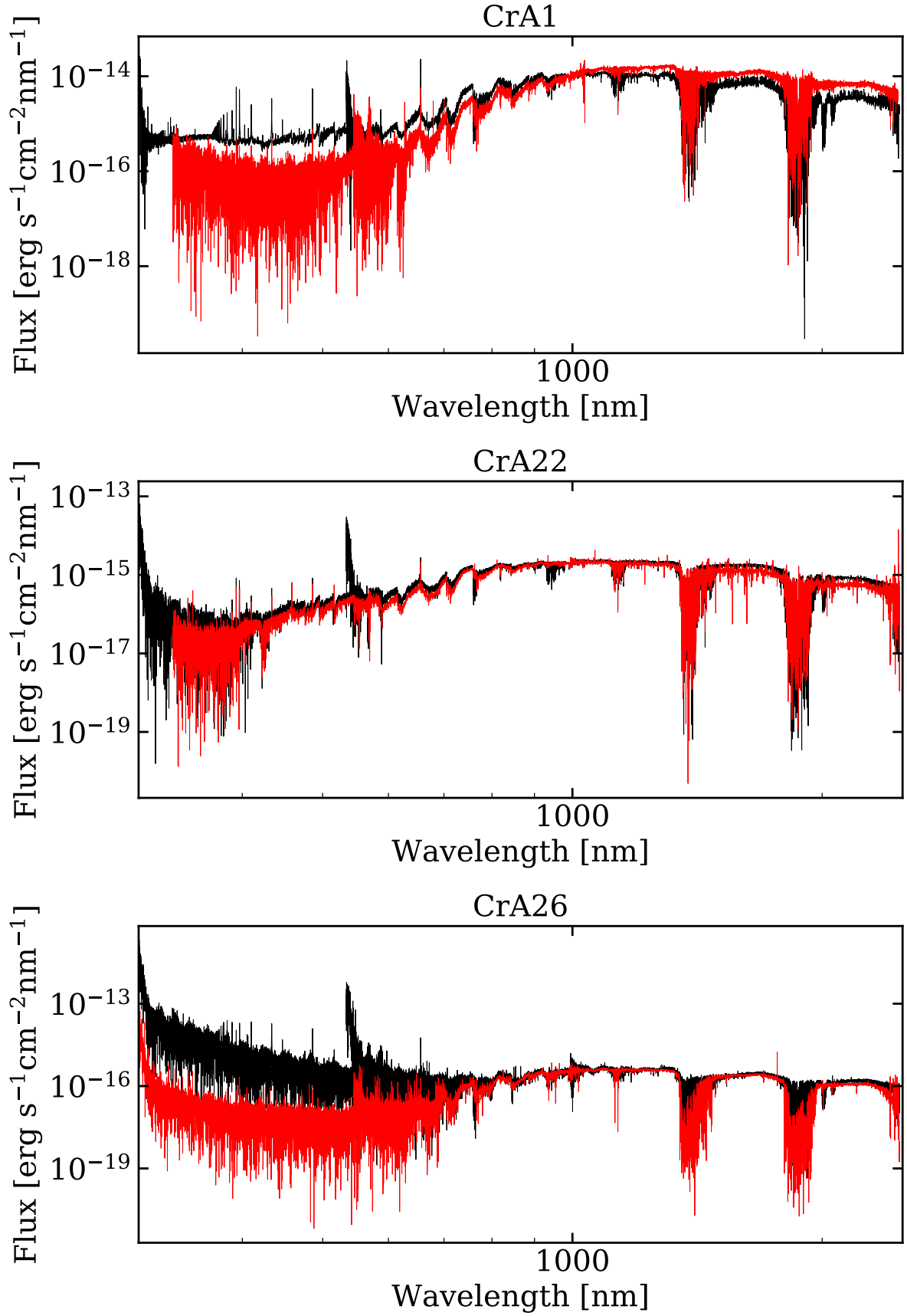
Fig. B.1. Spectra observed in our X-shooter programs (black) along with a template with the same SpT (red). The names of the sources are in the title of each subfigure. The absolute flux of each template was normalized to the flux of the observation at \lambda = 1 \mu\text{m} .
