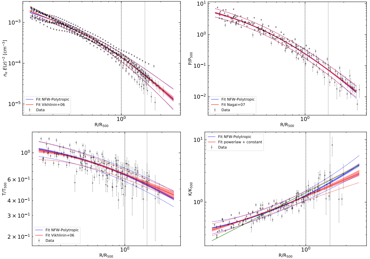
Fig. 3. Profiles of the (top) electron density and pressure, (bottom) temperature and entropy with, overplotted in blue, the joint fit obtained using the NFW-polytropic functional forms relating together the parameters c_{500} and \Gamma (see Table 3 and Sect. 3), and, in red, the functional form used in Ghirardini et al. (2019). The shaded area around the functional form represents the 1\sigma confidence level on the best fit, while the dashed lines represents the scatter around the best fit. The vertical dashed and dotted lines represent the location of R_{500} and R_{200} , respectively.
