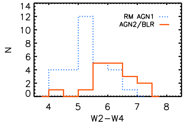
Figure 5. Distribution of the W2–W4 MIR colour of our sample of AGN2/BLR (red continuous line) and of the control sample of AGN1 whose M_{BH} have been measured via RM (blue dotted line).
