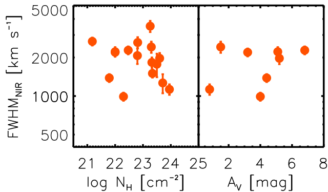
Figure 4. Left-hand panel: average FWHM of the BLR components of the NIR He I and Paβ lines of the AGN2/BLR as a function of the hydrogen column density N_H . Right-hand panel: same as the left-hand panel but as a function of the extinction A_V .
