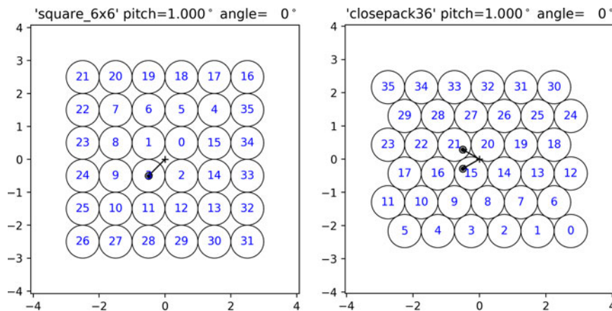
Figure 20. The two commonly used footprints: square_6x6 (left) and closepack36 (right). In this case, both have beam spacings (pitch) of 1.0^\circ and a position angle of zero. The scales are in degrees, and celestial north (west) is to the top (right) of both diagrams. The + symbol represents the optical axis of the reflector and the lines extending from this position ending in filled circles represent the pointing shift required to optimally interleave the footprint by using other observations to fill in the least sensitive parts. The square arrangement has larger intrinsic sensitivity variation but requires only one interleaving position, while the closepack arrangement is more uniform initially but requires two interleaving positions for improvement.
