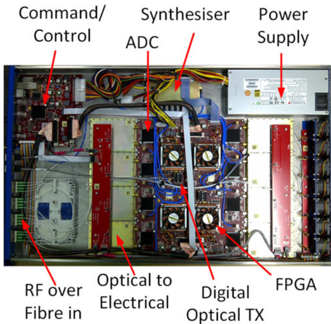
Figure 13. The Dragonfly digital receiver module, designed by CSIRO specifically for ASKAP. There are 12 per antenna.
