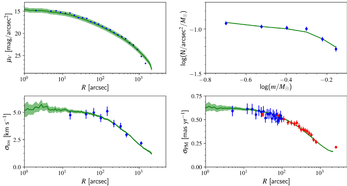
Figure 9. Fit of the grid of N -body models from Section 6 to the data set of case 3 (surface brightness, LOS velocities, HST and Gaia -like PM dispersion profiles, and mass function in an annular region between 250 and 350 arcsec). The mock data for the surface brightness profile (upper left), local stellar mass function (upper right panel), LOS velocity dispersion profile (lower left), and PM dispersion profile (lower right; \sigma_{\text{PM}} = (\sigma_{\text{PM},R} + \sigma_{\text{PM},T})/2 ) are shown with blue-filled circles, except the Gaia mock data shown in red. The 1\sigma confidence regions for the best-fitting model are indicated (when available) by the green-shaded area, and the median values are shown with green lines.
