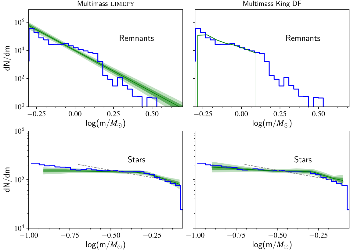
Figure 5. Inferred global mass function of dark remnants (upper panels) and visible stars (lower panels) from multimass model fits to the mock data from case 3. The results for the multimass LIMEPY models (Section 4.2) are shown in the left-hand panels, while those from the multimass models of Section 4.3 are shown in the right-hand panels. The 1\sigma and 2\sigma contours are shown with dark and light green-shaded regions, respectively, and the median values are shown with green lines. The true mass functions are shown with blue histograms. For comparison, we also show with a grey dashed line the best-fitting global mass function (when describing the global mass function as single power law in the range 0.2 < m < 0.8 M_\odot ) from the method of Section 6 based on a grid of N -body models.
