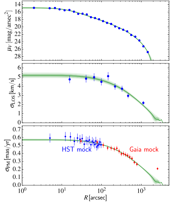
Figure 3. Fit of the three-component model from Section 4.1 to the data set of case 3 (fitting to surface brightness, LOS velocities, HST , and Gaia -like PMs). The mock data for the surface brightness profile (top panel), LOS velocity dispersion profile (middle panel), and PM dispersion profile (bottom panel) are shown with blue-filled circles, except the Gaia mock data shown in red. The most distant Gaia PM data point at \sim 3000 arcsec was not included in the fit. Median values at each R are shown with green lines, and the 1\sigma and 2\sigma contours are shown with dark and light green-shaded regions, respectively.
