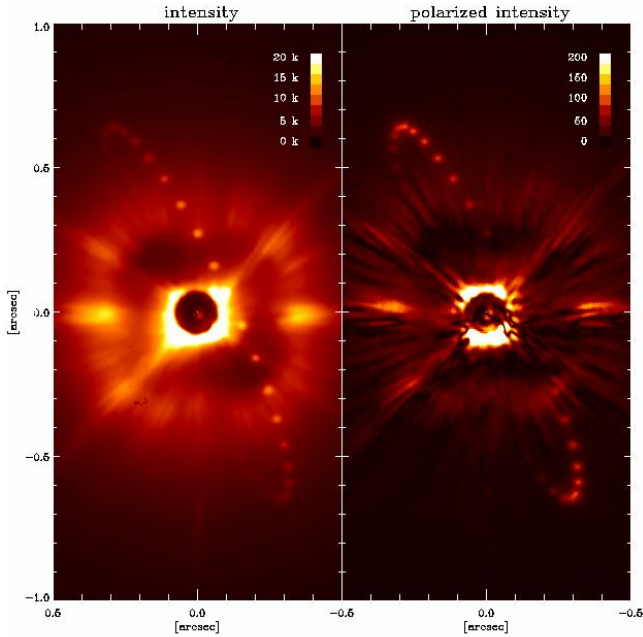
Fig. 2. Apparent positions of a model planet on a circular 80^\circ inclined orbit with r = 1 AU around \alpha Cen A in a typical coronagraphic intensity (left) and polarisation frame (right) at ten-day intervals. The brightness of the planet signal with respect to \alpha Cen A is exaggerated by a factor of 10^4 for the intensity and 10^3 for the polarisation. The relative brightness of the point for different phases is according to the model presented in Fig. 1.
