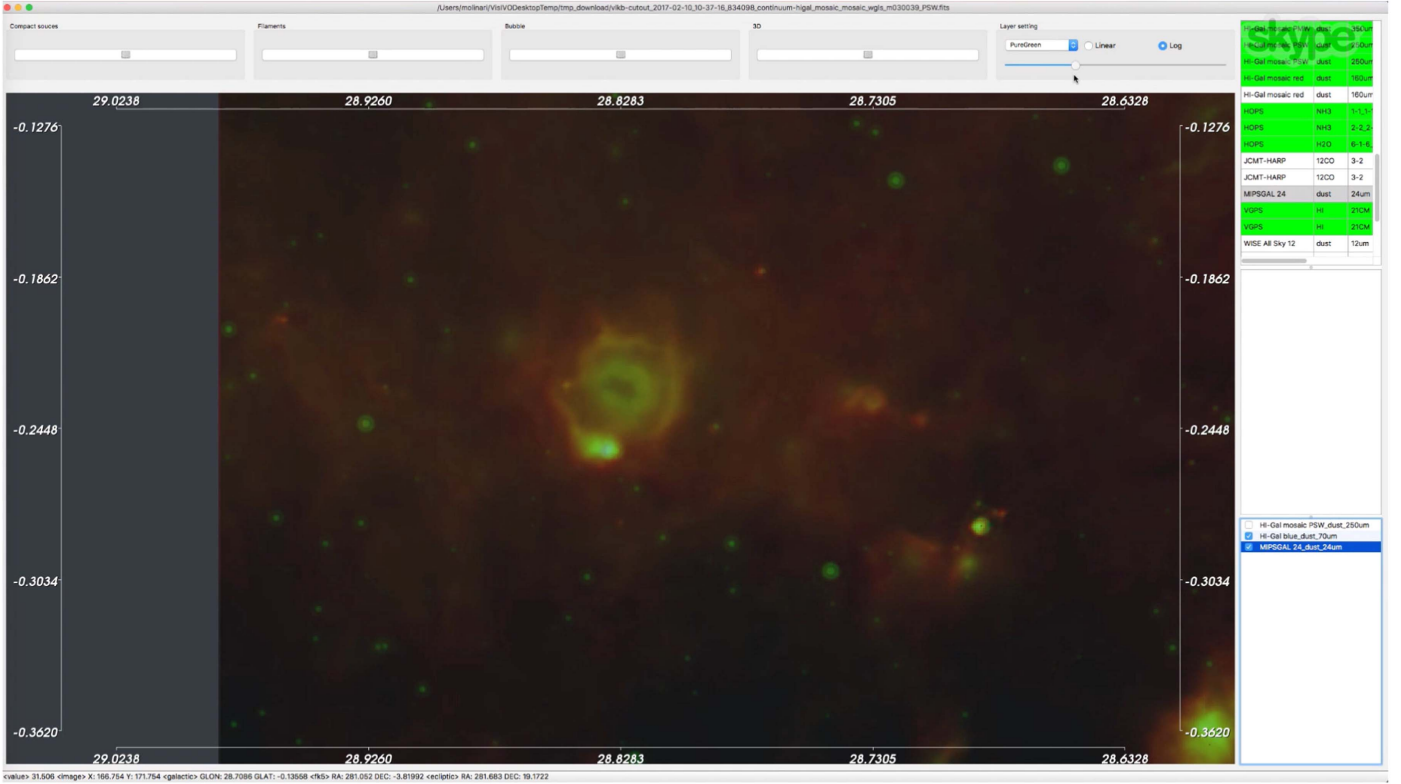
Figure 5. Bubble-like structure visualization. An Hi-GAL map at 70\ \mu\text{m} (with glow palette) superimposed on a 24\ \mu\text{m} MIPS GAL image (with pure green palette). (A color version of this figure is available in the online journal.)
