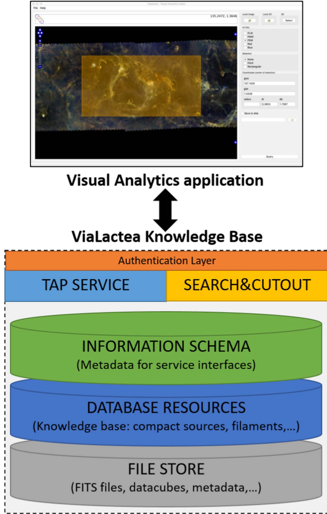
Figure 8. Visual Analytics application interacting with the ViaLactea Knowledge Base (VLKB). VLKB exposes data and metadata through the TAP service and the search & cutout service. (A color version of this figure is available in the online journal.)
