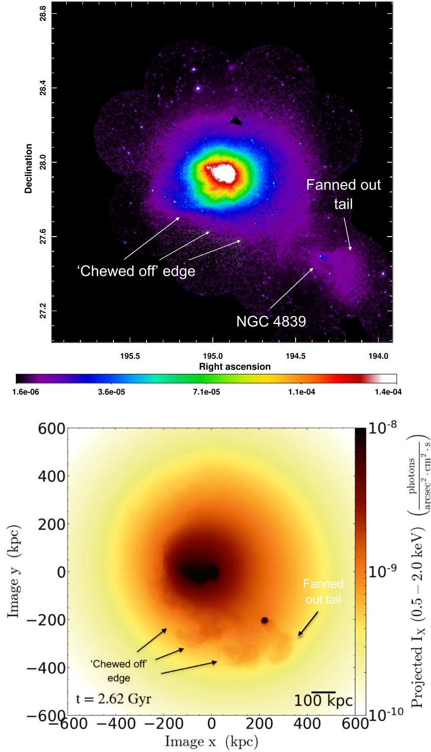
Figure 8. Top: image taken from Lyskova et al. (2019). An XMM-Newton image of the Coma cluster and the NGC 4839 group in the 0.5–2.5 keV energy. Bottom: X-ray photon intensity projection from the V1 simulation in Sheardown et al. (2018). The simulated image shows the overrun slingshot tail in action, and we see that the tail geometry matches the observed tail of NGC 4839. Physical scales are different as this simulation is not tailored to the Coma cluster. See Lyskova et al. (2019) for the tailored simulation of Coma and the NGC 4839 group.
