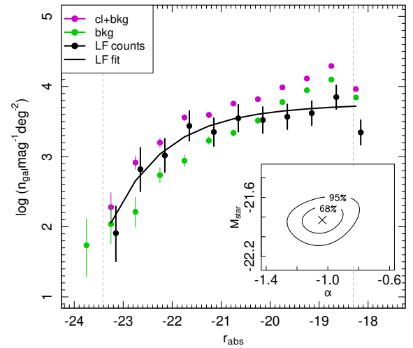
Fig. 3. Luminosity function for AK3 J091606.48-002328. The magenta dots represent the total counts coming from the region inside r_{200} ; the green dots represent the background counts coming from the background annulus only; and the black dots refer to the background subtracted counts, fitted by a Schechter function (black solid line) in the magnitude range delimited by the two grey vertical dotted lines. Inset: The confidence plot for the values of \alpha and M_* resulting from the fit; the contours at 1\sigma and 3\sigma are reported.
