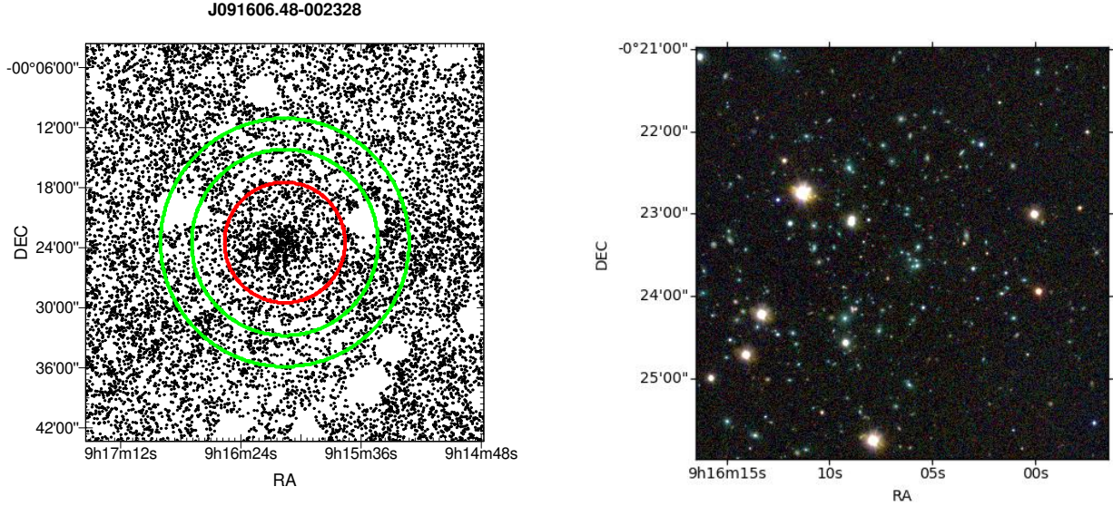
Fig. 2. AMICO-KiDS detection AK3 J091606.48-002328 or Abell 0776. Left panel: galaxy map of AK3 J091606.48-002328 (RA = 139.027, Dec = -0.3913, S/N = 9.68 , z = 0.37 , \lambda_* = 137 ): the region spans an area of \sim 50' \times 50' . The black dots represent the galaxies brighter than r_{\text{lim}} = 24.0 . The red circle encloses the central area within r_{200} \sim 6' ; and the two green circles delimit the area over which the background is estimated (in this case, an annulus with radii from 12' to \sim 18' ). The white holes in the galaxies distribution indicate masked areas. Right panel: colour composite ( g, r, i ) image relative to AK3 J091606.48-002328. The stamp shows a \sim 6' \times 6' region centred on the location identified by AMICO.
