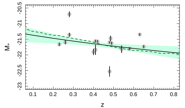
Fig. 10. Comparison between the evolution model for M_\star (Hennig et al. 2017) (green dashed line), used as a reference in the detection algorithm, and the observed M_\star evolution (grey dots). The 1\sigma confidence region (shaded area) of the best fit (black line drawn for \lambda_\star = 22.5 ) to our data is reported.
