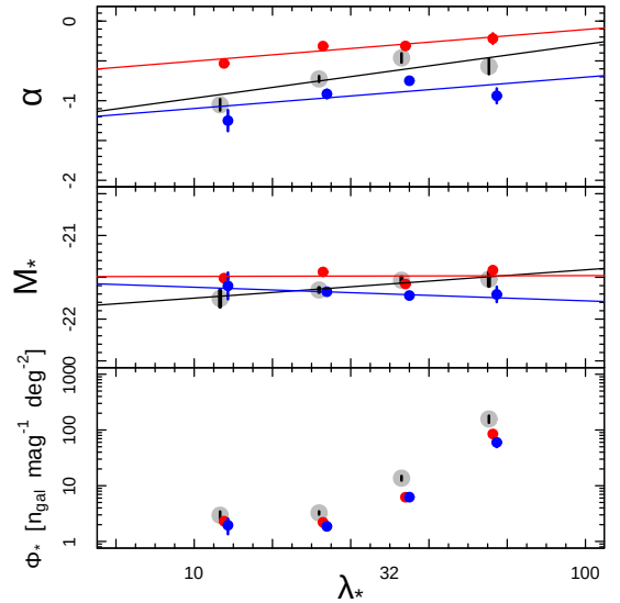
Fig. 7. Dependence of the Schechter fit parameters on richness/mass for all galaxies (grey dots), red galaxies (red dots), and blue galaxies (blue dots). The trend lines for all (black lines), red, and blue galaxies are overplotted, except for the lower panel where \Phi_* is increasing but with a clear non-linear trend.
