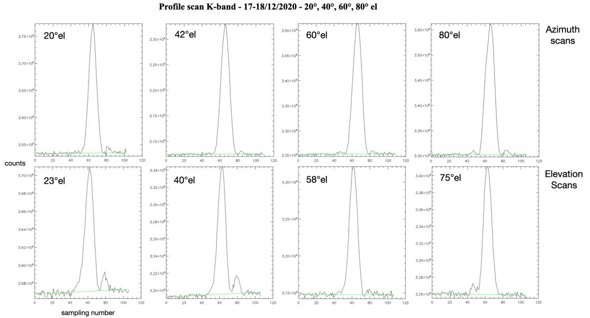
Figure 17: Profiles of the central scans of 3C84 in azimuth (top) and elevation (bottom) for 20°, 40°, 60° and 80° elevation (from left to right) using the data obtained on 17-18 December 2020.
