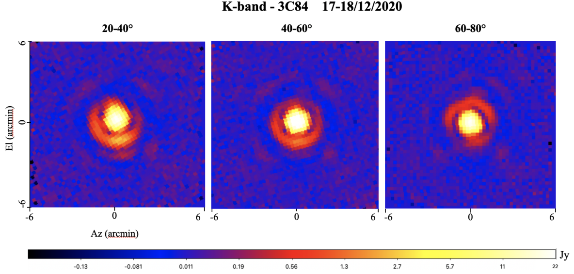
Figure 16: Az/EI maps of 3C84 in Jy at 20-40°, 40-60° and 60-80° of elevation obtained on 17-18 December 2020 at 18.7 GHz using the new M1-LUT, with a pixel resolution of 0.25'.
