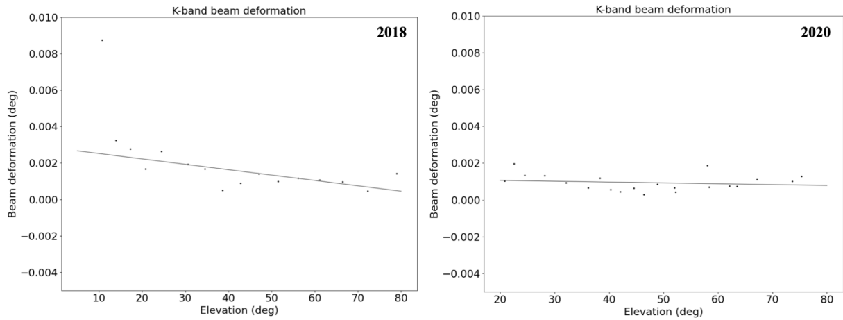
Figure 19: K-band beam deformation measured at 22 GHz in 2018 during the recommissioning (left) and in 2020 at 18.7 GHz (right).
