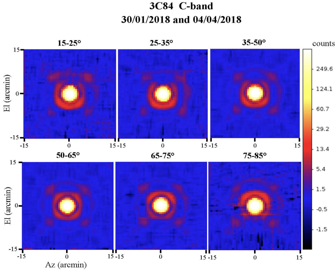
Figure 3: Az/El maps of 3C84 obtained at 7.2 GHz with the TP during the recommissioning (2018).
