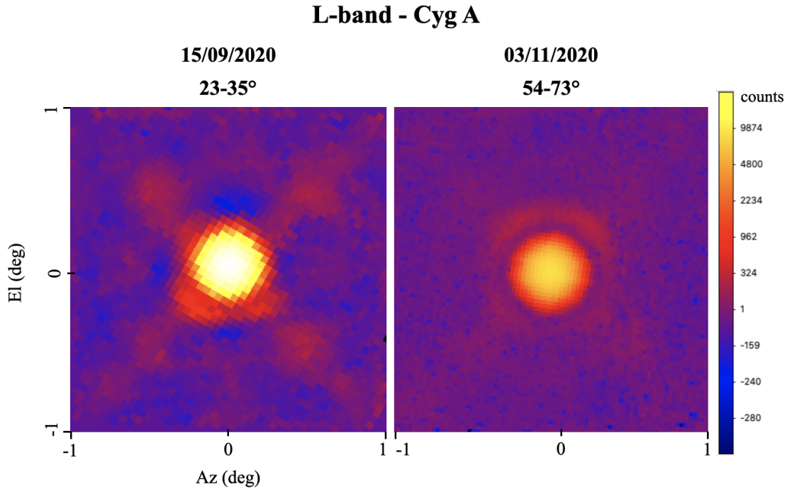
Figure 2: Az/El maps of Cyg A obtained at 1.5 GHz with SARDARA on 15 September and 3 November 2020. The difference in the pixel resolution is due to the difference in the parameters of the schedule: 4 passages/beam (left) and 8 passages/beam (right). The beam size is 0.24^\circ .
