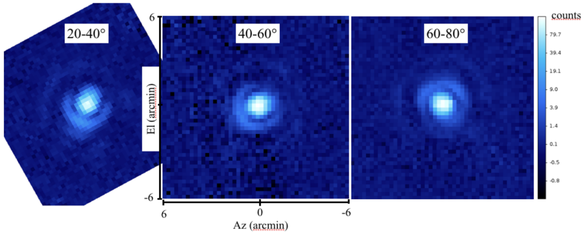
Figure 14: Az/El maps of 3C84 at 22.0 GHz in counts/beam at 20-40°, 40-60° and 60-80° of elevation (see Table 5) obtained in 2018 during the recommissioning, with a pixel resolution of 0.25' .
