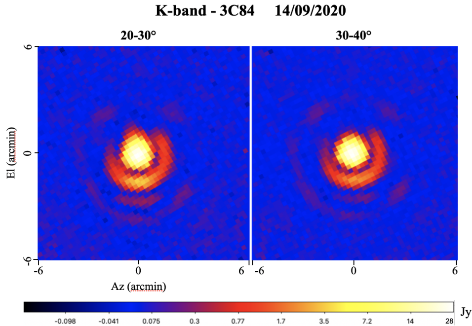
Figure 15: Az/El maps of 3C84 in Jy at 20-30° and 30-40° of elevation obtained on 14 September 2020 at 18.7 GHz, with a pixel resolution of 0.25'.
