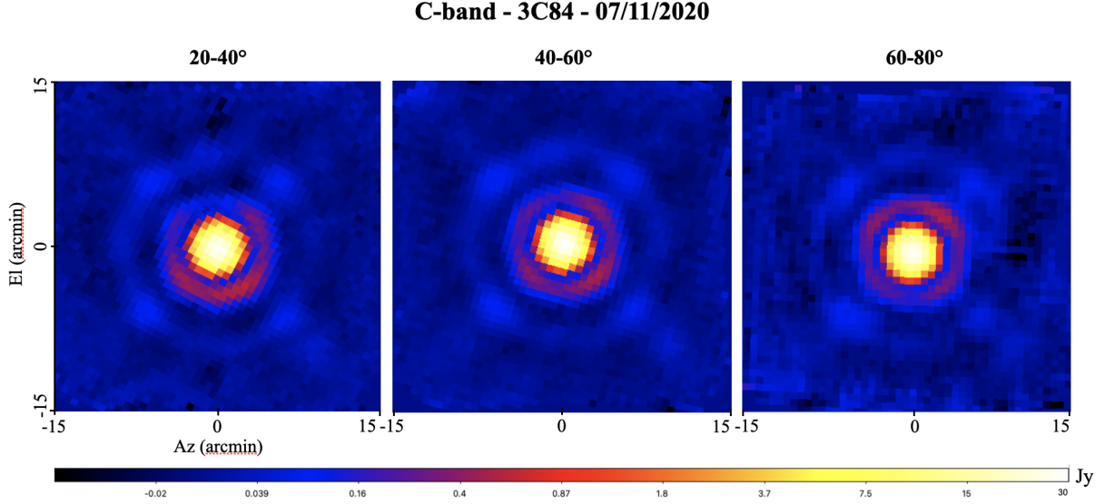
Figure 4: Az/EI maps of 3C84 obtained at 7.0 GHz with SARDARA on 7 November 2020.
