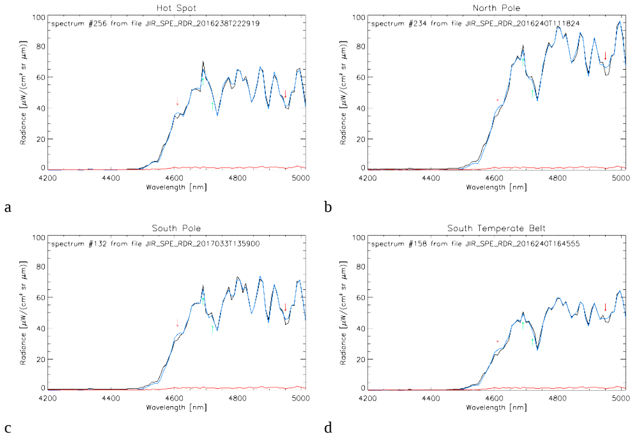
Figure 2. Examples of spectra fits produced by the retrieval code. Black: JIRAM data, blue: best fit spectrum, red: effective noise level, inclusive of forward model errors. The label in each panel identifies the JIRAM spectrum in the dataset stored at the NASA Planetary Data System [Noschese & Adriani, 2017]. The arrows show the locations of common occurrence of misfits described in the text.
