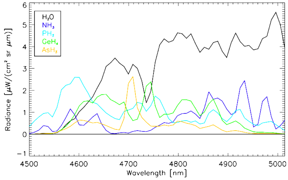
Figure 3. Expected effects on a bright spectrum ( \tau=0.1 , e.g.: fig. 2b) of gas variations corresponding to the 1\text{-}\sigma retrieval uncertainties quoted in the text. The different curves present the signal increase (not the absolute signal) obtained by decreasing (separately) the content of each gas of an amount corresponding to its 1\text{-}\sigma retrieval uncertainty. The horizontal black curve provides the zero level.
