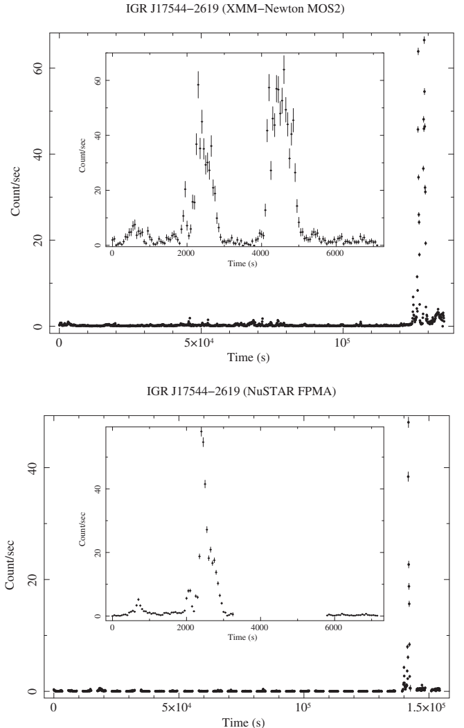
Fig. 1. Top: XMM-Newton MOS2 lightcurve of IGR J17544-2619 in the 0.5–10 keV energy band. The lightcurve has not been filtered for the high flaring background time intervals. The insert shows a zoom in the outburst of the source occurring towards the end of the observation and comprised of three distinct flares. The time bin of the main lightcurve is 100 s, while for the lightcurve in the insert we used a time bin of 50 s. The start time of the main lightcurve is 2015 March 20 at 06:02:34 UTC (57 101.2518 MJD), while the start time of the zoomed lightcurve in the insert is 2015 March 21 at 15:48:44 UTC (57 102.6588 MJD). Bottom: NuSTAR FPMA lightcurve in the 5–10 keV energy band. The time bin is 100 s and the start time is 2015 March 20 at 1:06 UTC (57 101.0458 MJD). The insert shows a zoom into the flaring part of the NuSTAR lightcurve (in this case the start and the bin times are the same as those of the insert in the top figure).
