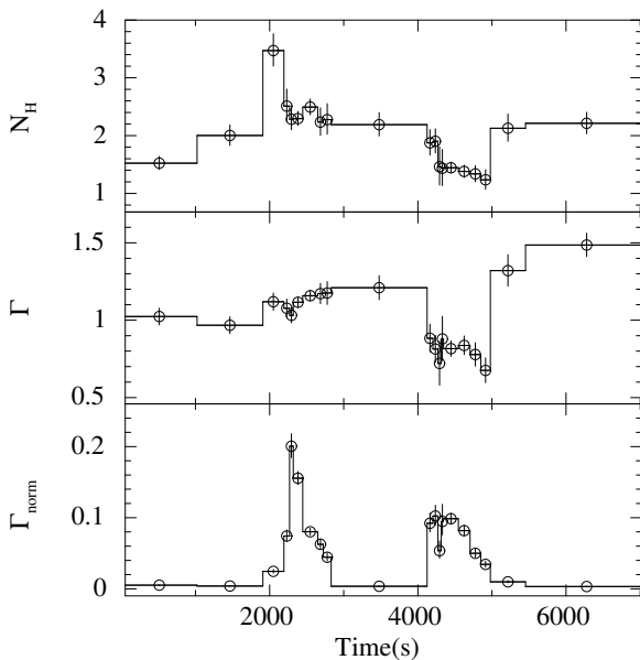
Fig. 6. Results obtained when the time-resolved XMM-Newton data alone are fitted with a simple absorbed power-law model. From the top to the bottom panel we show the absorption column density, the power-law photon index, and its normalization. As discussed in the text, it is evident that the most prominent spectral changes took place during the second flare (the first one being much fainter than the other two and occurring in this figure at approximately t = 500 s). The uncertainties on the x axis correspond to the integration times of the spectra 1–20 in Fig. 2.
