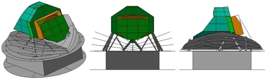
Fig. 8 Configuration of the instrument radiator on PLM
