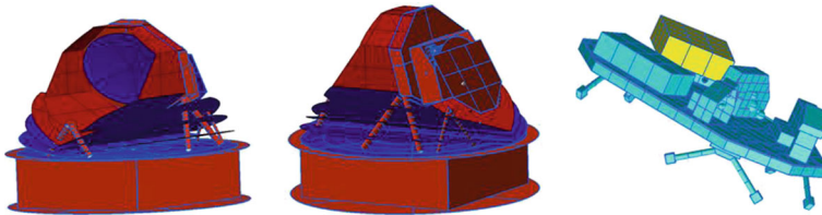
Fig. 14 EChO geometric model views. Left : the EChO S/C geometrical model. Middle : rear view with the cold radiator on top of the instrument box. Right : a view of the instrument optical bench geometric model with the main units
