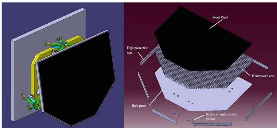
Fig. 9 CAD view of: Cold Radiator on the IOB ( left ), sandwich structure ( right )
