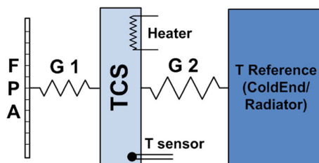
Fig. 6 Detector modules thermal control stage scheme
