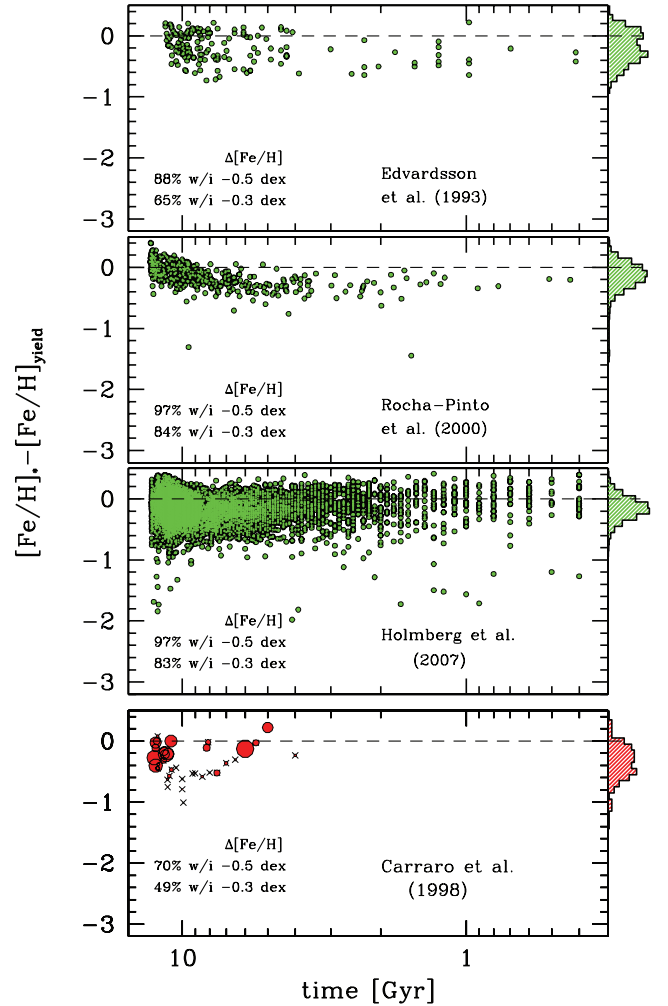
Figure 8. The observed metallicity distribution of stars in the solar neighbourhood. The displayed quantity is \Delta[\text{Fe}/\text{H}] = [\text{Fe}/\text{H}]_* - [\text{Fe}/\text{H}]_{\text{yield}} \equiv \log(Z_{\text{gas}}/Z) . Different stellar samples have been considered from the work of Edvardsson et al. (1993), Rocha-Pinto et al. (2000) and Holmberg et al. (2007), from top to bottom, as labelled in each panel. The lower panel displays the same trend for a sample of open stellar clusters, after Carraro, Ng & Portinari (1998). The different Galactocentric distance for these systems is indicatively marked by the dot size (i.e. the smallest the dot, the largest the distance from the Galaxy centre). For each distribution, the relative fraction of stars within a -0.3 and -0.5 dex \Delta[\text{Fe}/\text{H}] residual is reported in each panel. A cumulative histogram of the data is also displayed, along the right axis, in arbitrary linear units.
