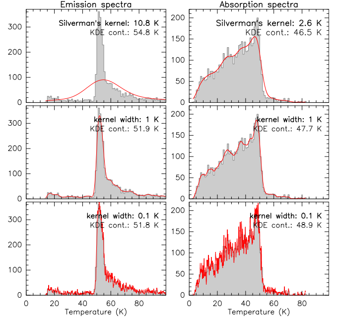
Fig. 3. Distribution of the intensities of emission-dominated (left panels) and absorption-dominated (right panels) spectra cases of Fig. 1. The red solid lines show the KDE for different kernel widths: (top) Silverman’s rule, (middle) kernel width of rms (=1 K), and (bottom) kernel width one tenth of the rms (=0.1 K). The continuum level determined as the position of the maximum of the KDE is indicated in each panel.
