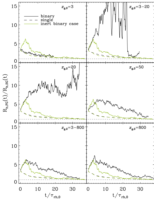
Figure 1. Time evolution of the ratio of the half-mass radii of FG stars to SG stars. Models with x_{g,0} = 3, 3-20, 20, 50, 3-800 , and 800 are shown in different panels. The solid and dashed lines represent the ratio of half-mass radii for binaries and single stars, respectively. For the inert binary model (green lines), stars with 2m are plotted for comparison with the evolution of binaries. The horizontal dotted line at R_{h,\text{FG}}/R_{h,\text{SG}} = 1 indicates the completion of the spatial mixing.
