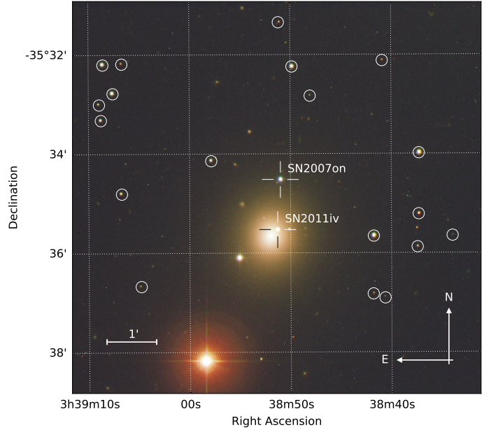
Fig. 1. Composite image of NGC 1404 with the positions of SN 2007on, SN 2011iv, and a number of local sequence stars indicated.
