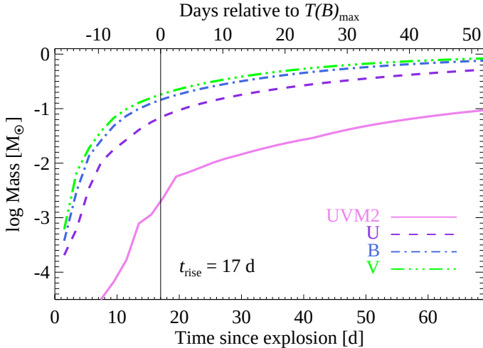
Fig. E.1. The amount of SN Ia ejecta mass probed by the emission contained within the uvm2 , U , B , and V bands as a function of days past explosion. These calculations are based on the DD model 5p0z22.18b. The masses are calculated by first averaging the opacity across the filter range, and then the total mass at this opacity is integrated from infinity down to an optical depth of unity.
