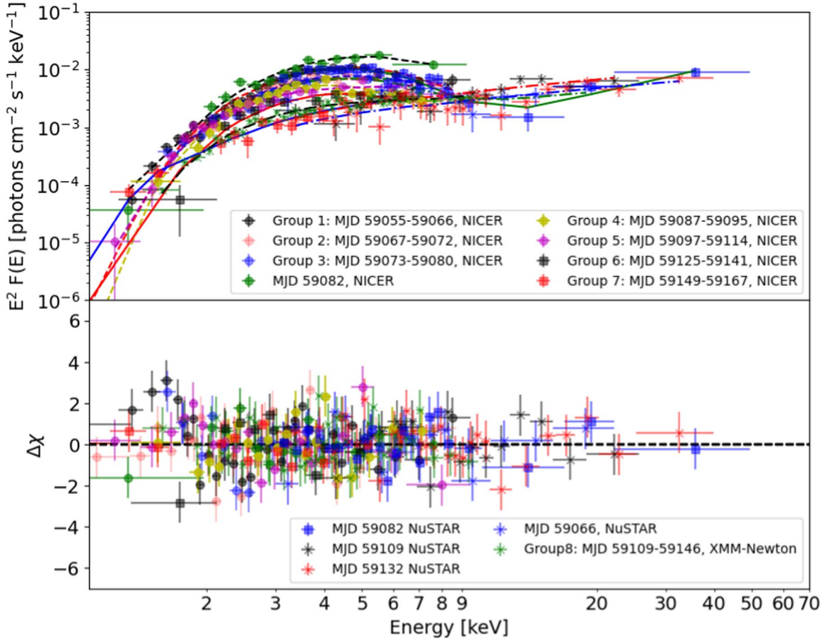
Figure 8. Top panel: absorbed ( N_H = (5.5 \pm 0.3) \times 10^{22} \text{ cm}^{-2} ) unfolded (deconvolved) pulsed energy spectra of PSR J1846–0258 in the aftermath of the 2020 outburst using NICER, NuSTAR, and XMM-Newton observations (see text). For display purposes, the NICER spectra were separated into seven groups, where in each group the spectra were stacked using the addspec tool (for the observation date ranges indicated in the legend). Similarly, the three XMM-Newton spectra were also combined. However, for spectral fitting we used the original spectra for each observation (see Table 1). Each spectrum was fit with an absorbed blackbody plus power-law model with the column density tied between the different observations. The results clearly demonstrate the gradual fading of the thermal component (below 10 keV) during the outburst, while the power-law component (above 8 keV) remains unchanged. The detailed best-fit parameters are reported in Table 1. The residuals of the best-fit model are also shown in the bottom panel of the figure.
