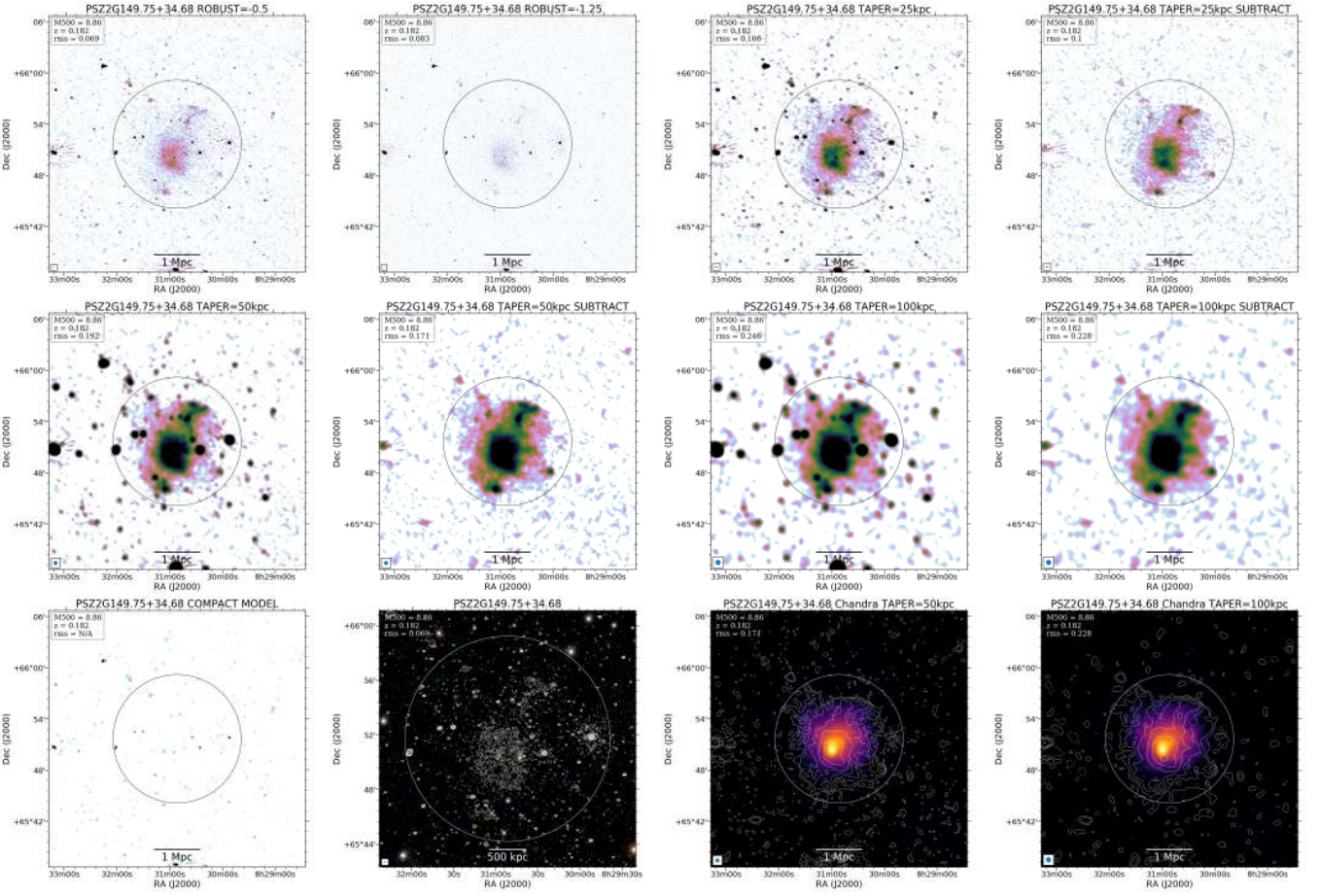
Fig. 3. Example of the set of images that we produced for each object in our sample. The displayed cluster is PS22 G149.75+34.68, and the reported panels show (from left to right and from top to bottom) the reference image (robust=-0.5), the high-resolution image (robust=-1.25), taper 25, 50, and 100 kpc images with and without discrete sources, the clean model components used for the source subtraction, contours from the reference radio image starting from 3\sigma overlaid on an optical image (Pan-STARRS g,r,i ), and taper 50 and 100 kpc discrete-source-subtracted contours starting from 2\sigma overlaid on an X-ray image ( Chandra or XMM-Newton ). Contours are always spaced by a factor of 2. The beam is shown in the bottom-left corner, and the mass ( M_{500} , in \times 10^{14} M_{\odot} units), redshift ( z ), and image noise (rms, in mJy beam ^{-1} units) are reported in the top-left corner. The circle denotes r_{500} and is centered at the coordinates reported in the PS22 catalog. The images are available at full resolution as well as in FITS format on the project website, https://lofar-surveys.org/planck_dr2.html .
