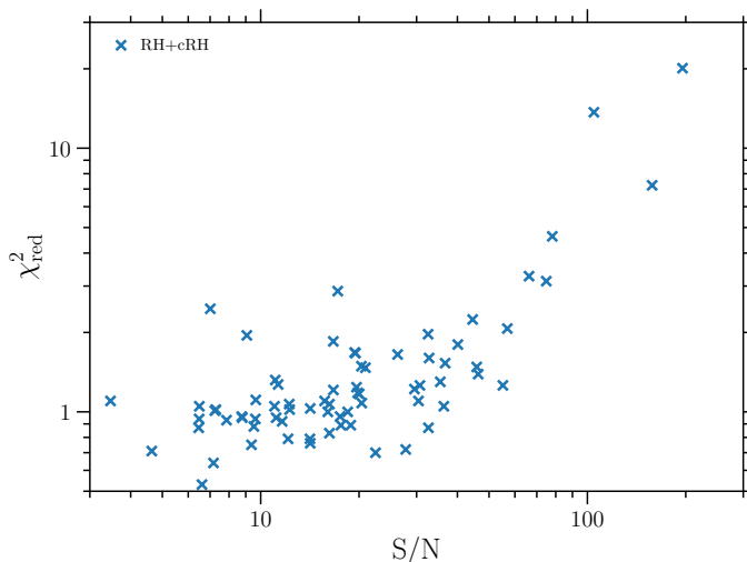
Fig. 7. \chi^2_{\text{red}} vs. S/N (i.e., the ratio between the integrated flux density and its fitting uncertainty) for the radio halos and candidate radio halos in our sample. The positive trend indicates that deviations from the exponential model become evident only for the halos that are detected with sufficient significance.
