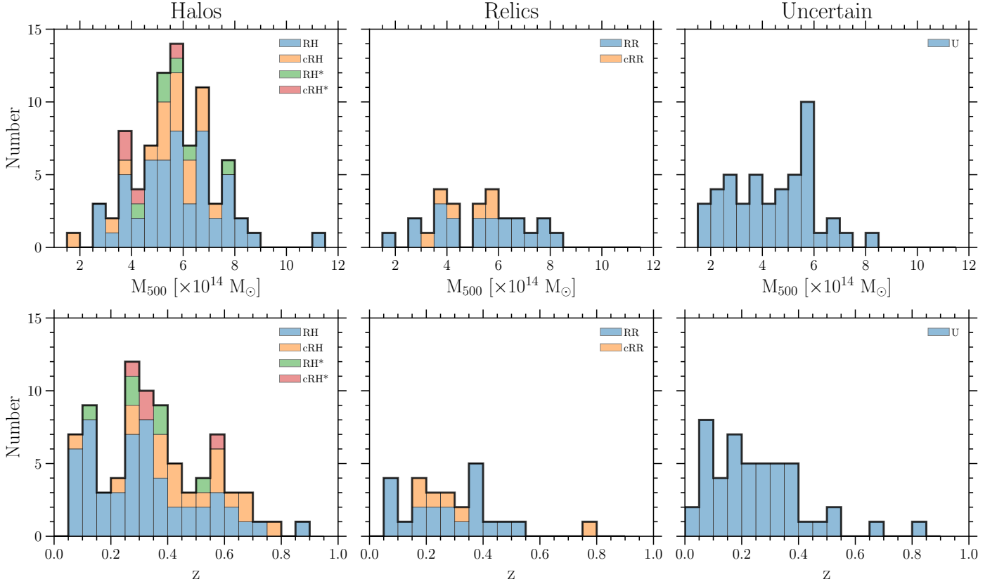
Fig. 9. Histograms of the mass ( top panels ) and redshift ( bottom panels ) distribution for the main categories of objects classified in this work.
