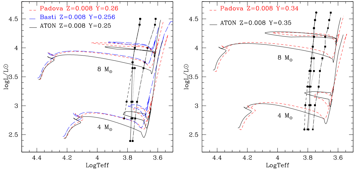
Figure 2. The evolutionary path in the HR diagram of a 4 M_{\odot} and 8 M_{\odot} model calculated with the ATON code (black solid line) is compared to that from other data bases: Basti (long dashed blue line) and Padova (short dashed red lines) for Y = 0.25 (left-hand panel) and Y = 0.35 (right-hand panel, see the text). The FRE (dot dashed black line), FORE (dotted black line), FBE (solid black line) and FOBE (short dashed black line) derived in Carini et al. (2014) are also shown.
