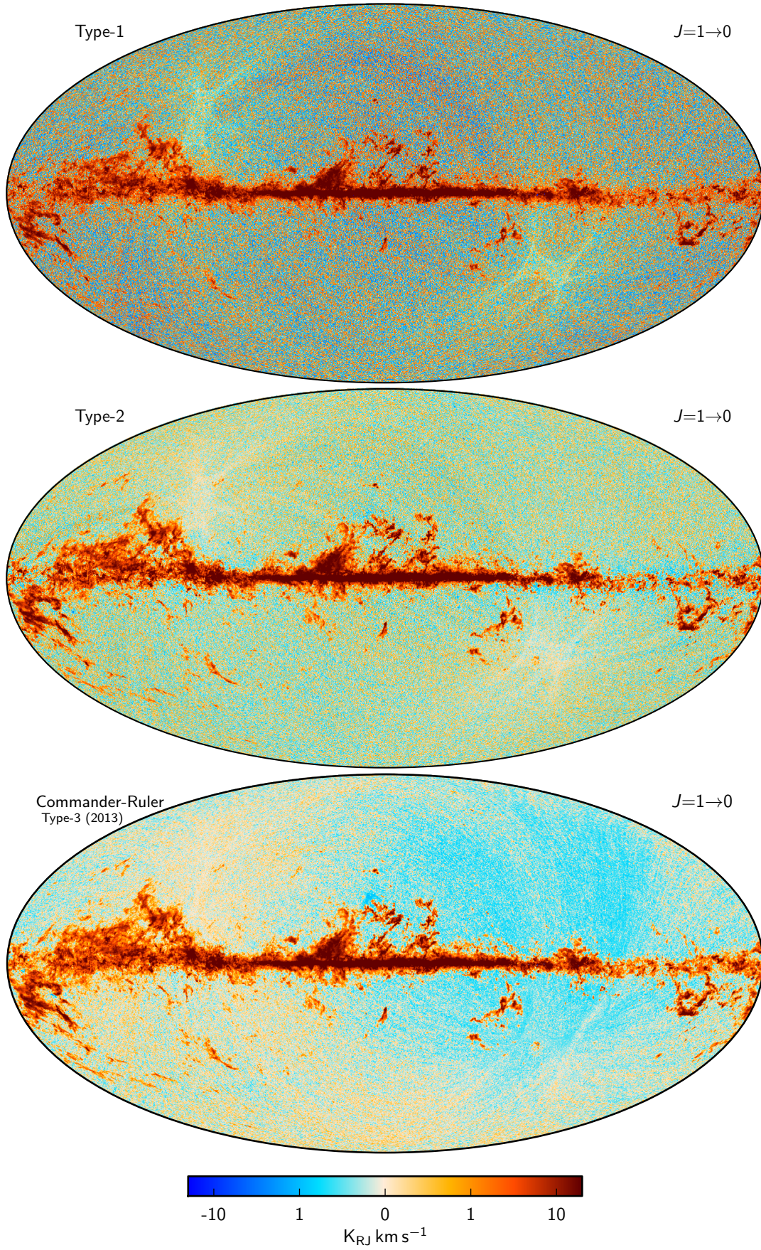
Fig. 30. High-resolution CO J=1 \rightarrow 0 maps derived from the 2015 Planck sky maps with two different algorithms, denoted Type-1 (top row) and Type-2 (middle row); and derived from the 2013 Planck sky maps with Commander-Ruler (bottom row). Details can be found in Planck Collaboration XIII (2014) . All maps are smoothed to a common resolution of 15' FWHM.
