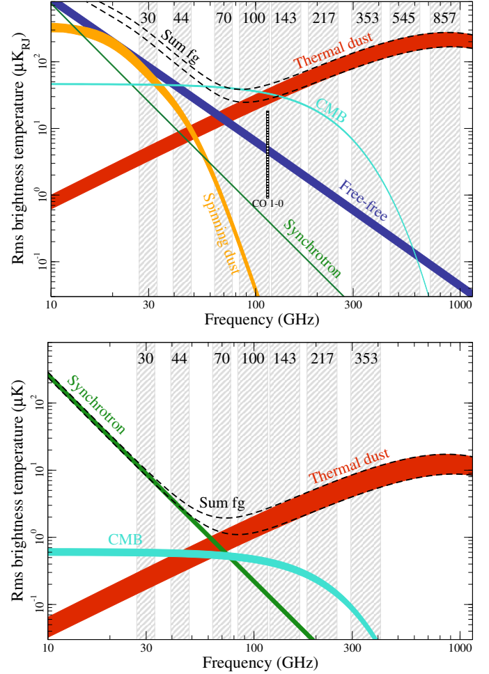
Fig. 51. Brightness temperature rms as a function of frequency and astrophysical component for temperature ( top ) and polarization ( bottom ). For temperature, each component is smoothed to an angular resolution of 1^\circ FWHM, and the lower and upper edges of each line are defined by masks covering 81 and 93 % of the sky, respectively. For polarization, the corresponding smoothing scale is 40' , and the sky fractions are 73 and 93 %. Note that foreground rms values decrease nearly monotonically with sky fraction, whereas the CMB rms is independent of sky fraction, up to random variations.
