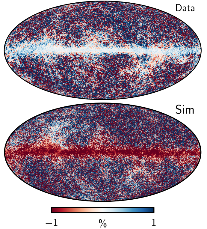
Fig. 5. Fractional difference maps on the form (d_{143-\text{ds}1} - d_{143-\text{ds}2})/d_{143-\text{ds}1} , as evaluated from the real data ( top ) and from the FFP8 simulation ( bottom ), both smoothed to 40' FWHM. The 1 % difference observed along the Galactic plane is caused by a mismatch between the measured bandpass profiles (which are used to construct the FFP8 simulations) and those corresponding to in-flight observations. See Sect. 4.3 for further discussion, and Sect. 5.3 for explicit corrections.
