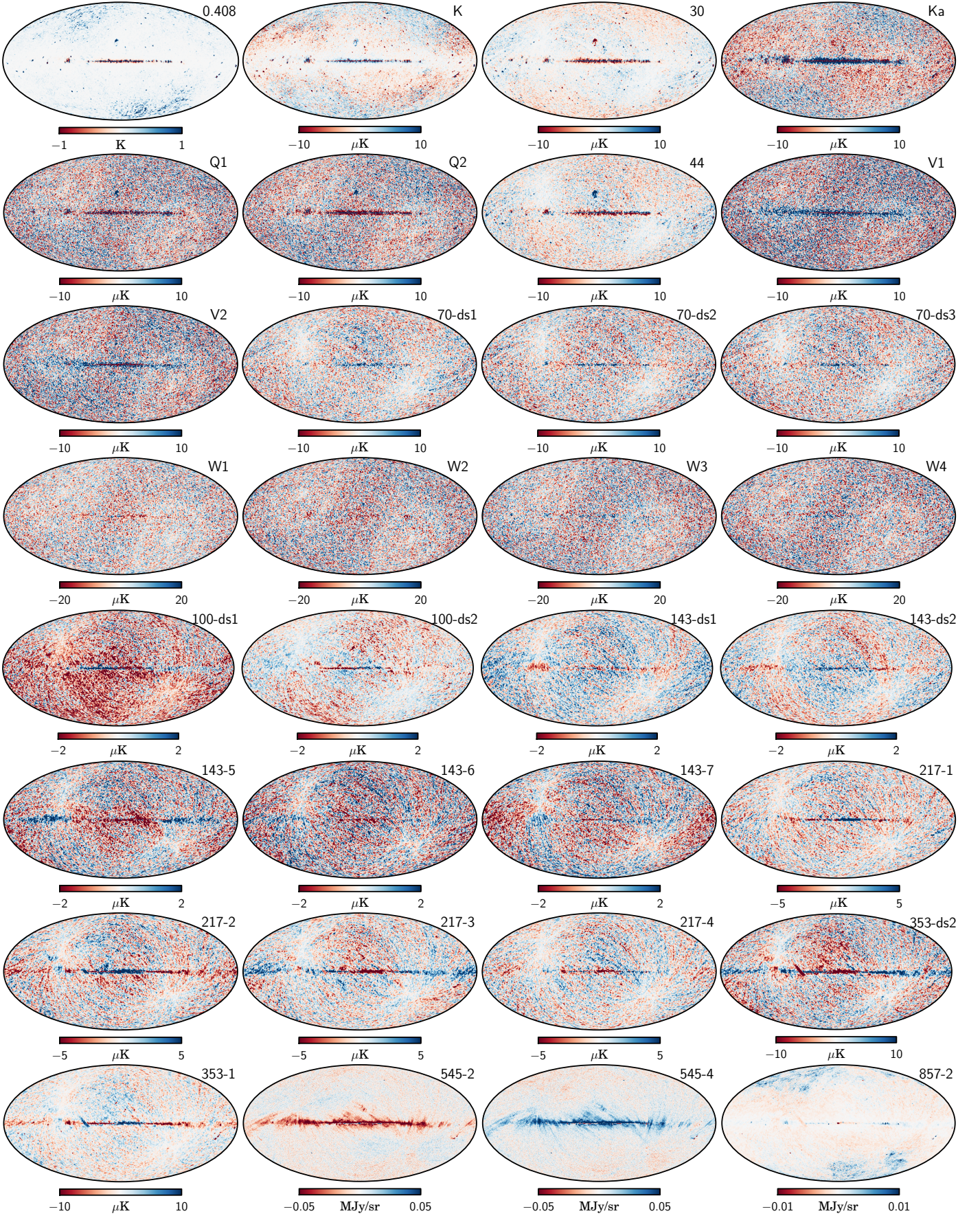
Fig. 21. Residual maps, d_\nu - s_\nu , for each detector data set included in the baseline joint Planck , WMAP, and 408 MHz temperature analysis. All panels employ linear colour scales.
