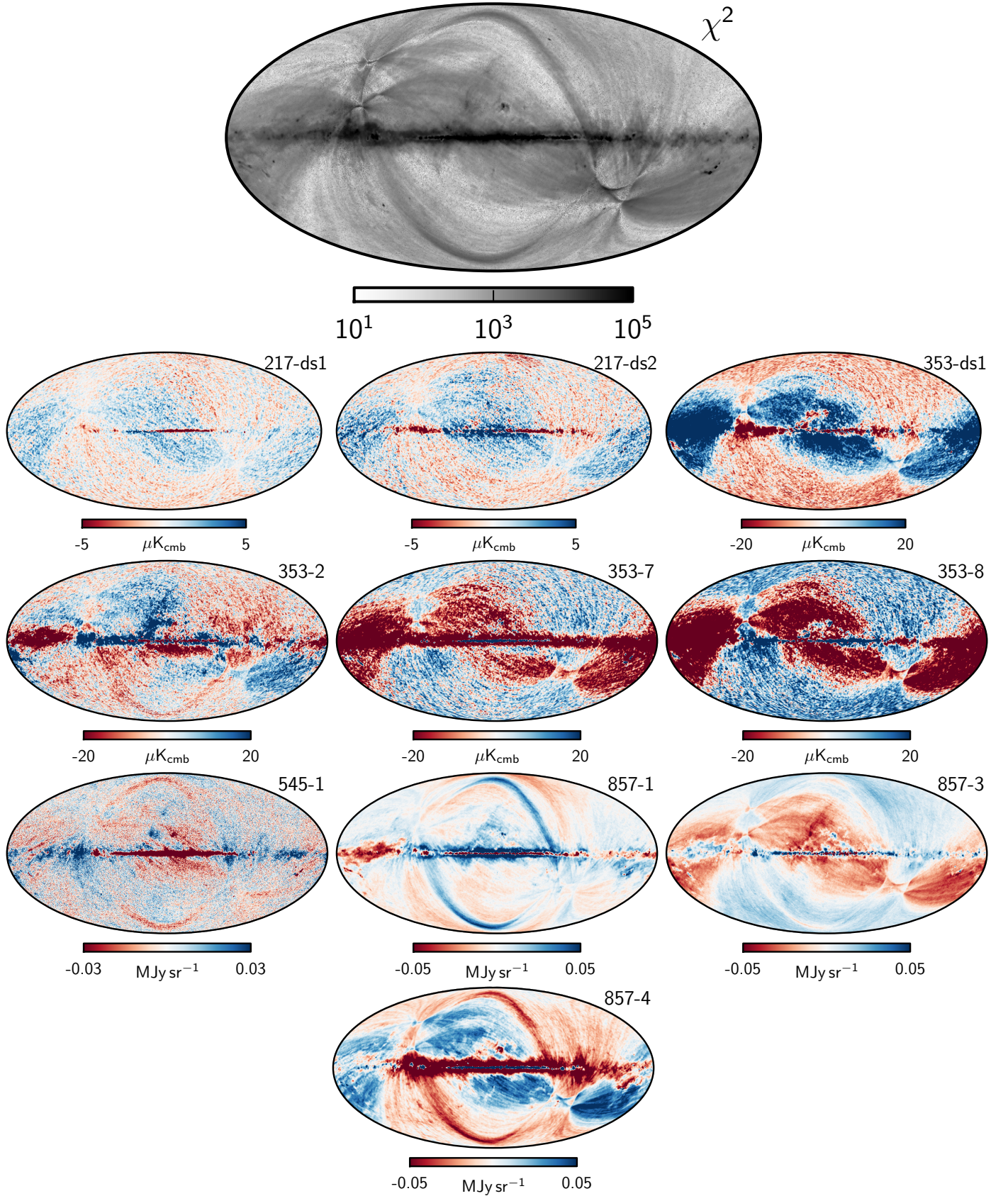
Fig. 2. \chi^2 (top) and residual maps, d_\nu - s_\nu (bottom), for a Commander analysis that includes all Planck channel maps. These residual maps correspond to channels that are rejected from the baseline analysis due to instrumental systematics. No regularization noise has been added to the high-frequency channels in this case. The sharp ring-like features at high Galactic latitudes correspond to far sidelobe residuals; the broad features extending between the north and south ecliptic poles correspond to destripping errors; and the Galactic plane features correspond to calibration, bandpass, and modelling residuals.
