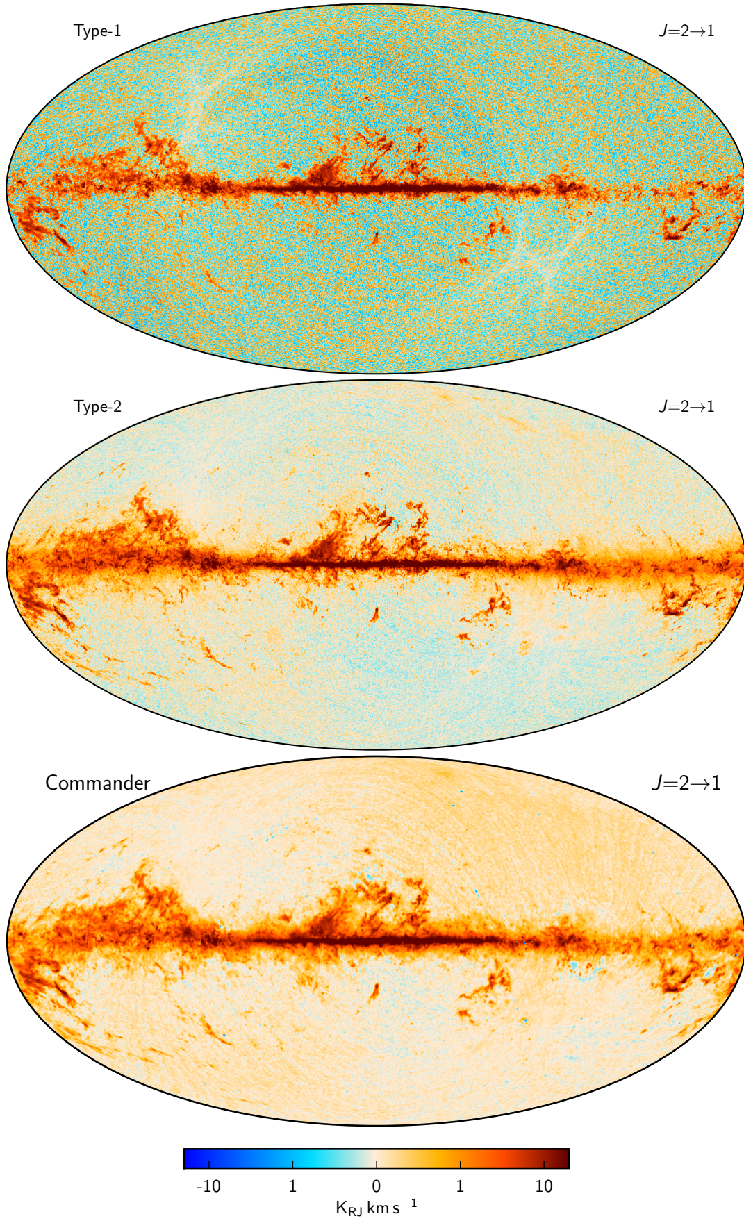
Fig. 31. High-resolution CO J=2\rightarrow1 maps derived from the 2015 Planck sky maps with three different algorithms, denoted Type-1 (top row), Type-2 (middle row) and Commander (bottom row), see Planck Collaboration XIII (2014) for details. All maps are smoothed to a common resolution of 15' FWHM.
