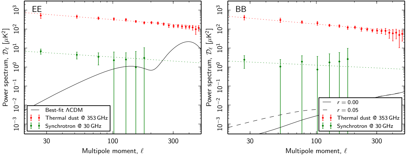
Fig. 44. Angular EE (left panel) and BB (right panel) power spectra for polarized synchrotron (at 30 GHz) and thermal dust emission (at 353 GHz), evaluated with 1^\circ FWHM apodization and including a total effective sky fraction of 73 % of the sky. The dashed lines show the best-fit power-law models to each case, and the solid black lines shows the best-fit \Lambda CDM power spectrum as fitted to temperature observations only (Planck Collaboration XI 2015; Planck Collaboration XIII 2015). The dashed black line in the BB panel shows the spectrum for a model with a tensor-to-scalar ratio of r = 0.05 .
