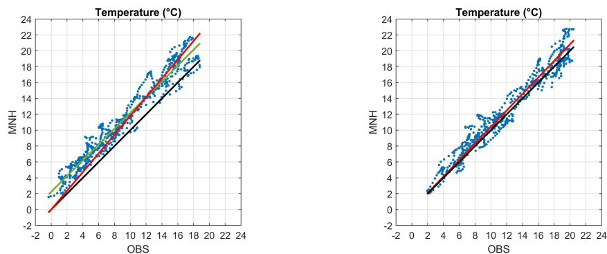
Figure 5. DAY TIME - Left: Temperature for NOT with the 2011 sample of 20 nights. The green curve is the fit showing an off-set of 2.24 degrees ( \text{BIAS}=2.18^\circ , \text{RMSE}=2.47^\circ and \sigma=1.17^\circ ). Right: Temperature for TNG and the 2011 sample of 20 nights ( \text{BIAS}=0.61^\circ , \text{RMSE}=1.27^\circ , \sigma=1.12^\circ ).
