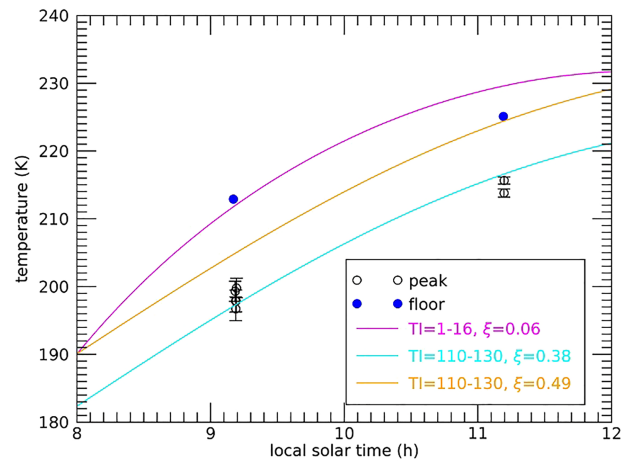
Figure 4. Comparison between theoretical (solid lines) and observed (black bars) temperatures for the peak in the Haulani crater. The thermal inertia derived from the model is 120 \pm 10 \text{ J} \cdot \text{m}^{-2} \cdot \text{s}^{-1/2} \cdot \text{K}^{-1} . The blue dots refer to the floor (see text), and the magenta line refers to a thermal inertia equal to the Ceres's average. For the comparison with the average thermal inertia of Ceres a roughness \xi = 0.06 was assumed in order to have temperatures comparable with the floor points. The error bars of the floor points are small and are not visible at the scale of the picture.
