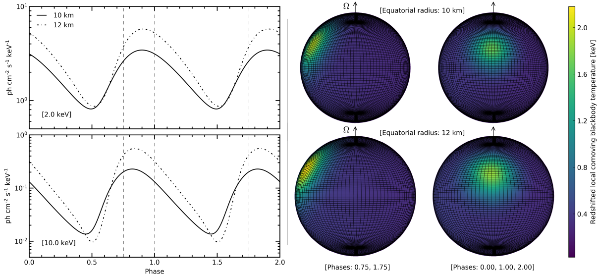
Figure 5 We illustrate the response of monochromatic pulse profiles to variation of the (circumferential) equatorial radius, whilst all other parameters are fixed at the values implemented in Figure 4. We use the realistic exterior spacetime described in Figure 4. The two synthetic stars shown are of equal gravitational mass and spin frequency, but have equatorial radii of 10 km and 12 km; these stars require distinct EOS models to exist. The pulse profiles are clearly sensitive to the equatorial radius, and it is the need to detect such differences that drives the design requirements for eXTP.
