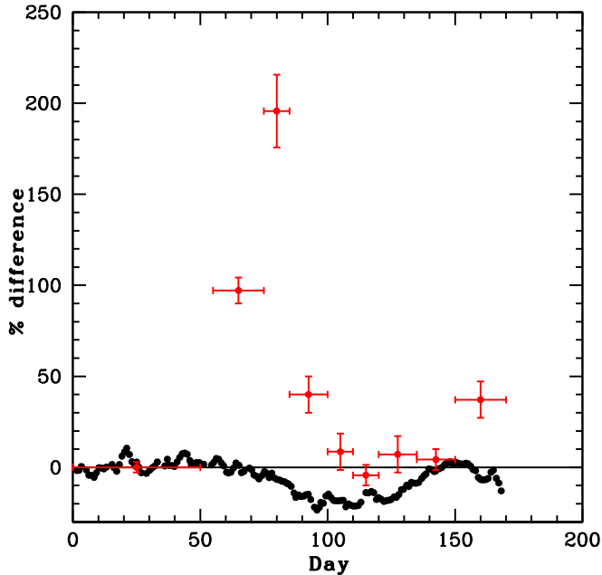
Figure 2. NGC 5548 light-curve. The black points show the percentage deficit in the C IV flux (reproduced from Figure 1(e) of Paper IV). This shows the onset of the anomaly around day 75 of the campaign. The red points show the percentage excess in the Swift count rate at \approx 0.55 keV (as in Figure 1). We see that the soft excess increases before the start of the anomaly, peaks during the period of anomaly and then declines.
