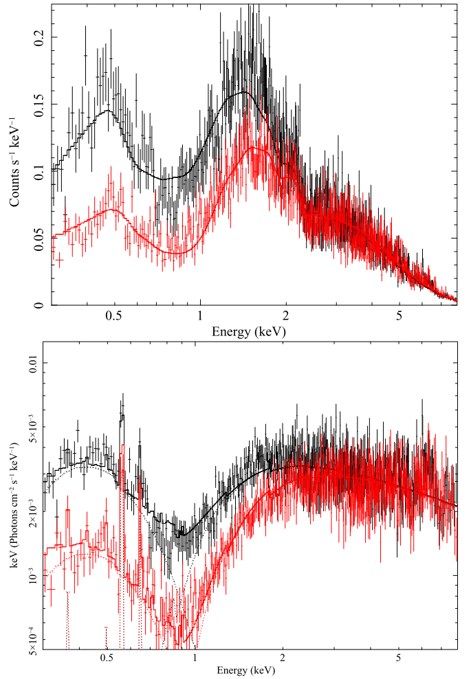
Figure 3. Top: Swift spectra: anomaly (black) and pre-anomaly (red) fit with an absorbed power law plus a blackbody model. An additional scattered component is also included. Bottom: the Ef(E) intrinsic spectra (without folding in the instrument response); the three model components are shown as dotted lines.
