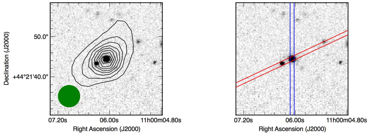
Fig. 7. (Left): Subaru/HSC z -band image in gray scale overlaid with the FIRST radio data in contour. The central object in this figure is J1100+4421. Beam size of the FIRST image (5.4 arcsec) is shown at the left-bottom part of the figure in green. (Right): The slits of the FOCAS and GMOS observations are shown in blue and red, respectively.
