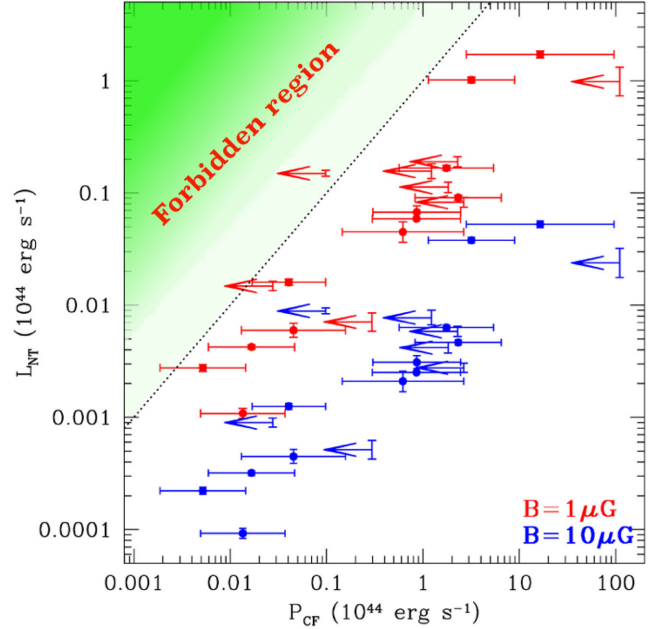
Figure 2. Correlation between L_{NT} and P_{CF} for our mini-halo cluster sample. The red and blue points were calculated assuming B = 1 and 10 \mu G , respectively. The black dotted line represents the 1:1 relation. The upper side of 1:1 relation is the forbidden region, where L_{NT} > P_H \sim P_{CF} .
