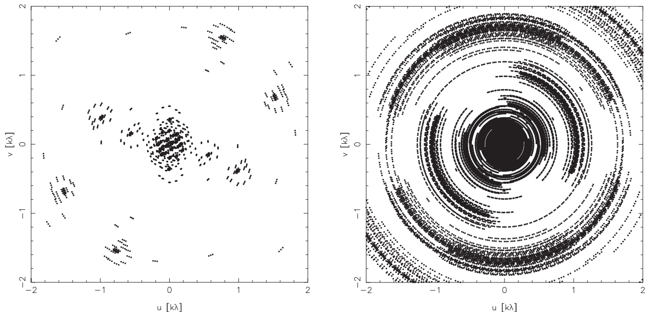
Figure 3. Left panel: the uv coverage obtained with an 11 min snapshot. Right panel: the improved uv coverage gained when combining 27 snapshots (297 min). In each case the uv range is limited to \pm 2 k \lambda (10 km).
