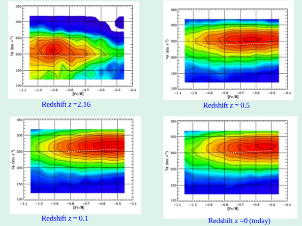
Fig. 5. Distribution V_{\phi} - [\text{Fe}/\text{H}] of the simulated “thick disk” in the “solar” neighborhood, 6 \text{ kpc} < R < 8 \text{ kpc} . The white dashed lines show the resulting linear best fit
