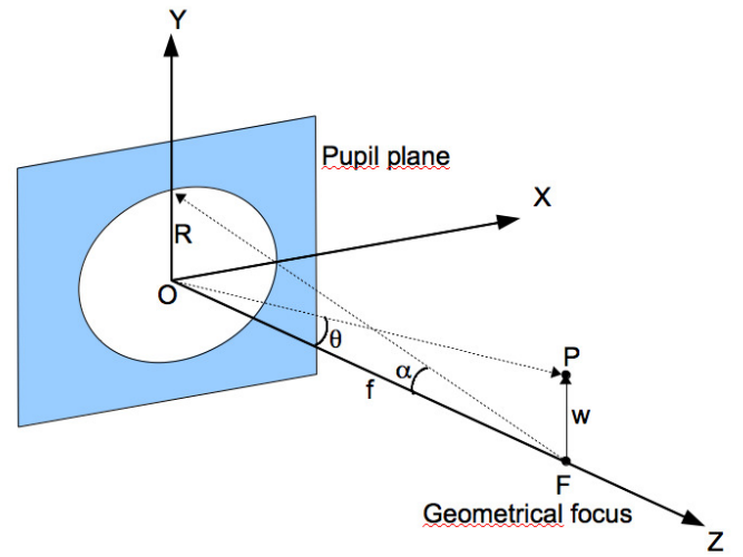
Fig. 2. Illustration of the notation used in determining Eq.(9). P is a point near the focus, F, f is the focal length, and R is the pupil radius. w represents the radial coordinate in the focal plane.
