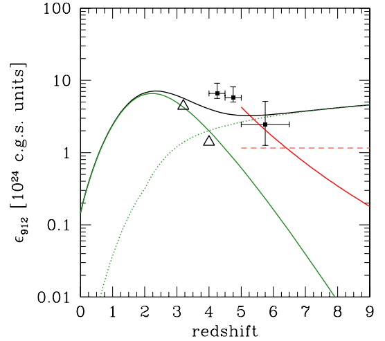
Fig. 1. Highest emissivity at the H I Lyman limit vs. redshift. The red solid curve at z \geq 5 is our benchmark case, consistent with the XRB limit J_{1.5 \text{ keV}}^{\text{obs}} \leq 1.9 \times 10^{-27} \text{ erg cm}^{-2} \text{ s}^{-1} \text{ Hz}^{-1} \text{ sr}^{-1} . This value accounts for sources at z \lesssim 5 below the Chandra flux limit, estimated from the XRB synthesis model of Gilli et al. (2007). The dashed line shows the extreme case of a constant comoving redshift evolution of the AGN emissivity. The black line is the emissivity employed in the UV background model of Haardt & Madau (2012), with galaxies (dotted green line) and AGNs (solid green line) shown separately. The black data points are the AGN emissivity as estimated by Giallongo et al. (2015), while open triangles are data from Masters et al. (2012).
