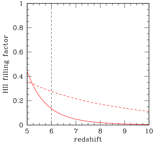
Fig. 2. Highest volume filling factor of H II vs. redshift. Curves as in Fig. 1. The dashed vertical line marks a fiducial reionisation redshift, z = 6 . In our benchmark case the contribution to H II reionisation from AGNs is lower than 13%.
