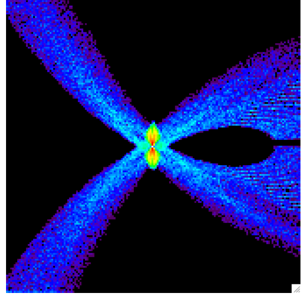
Figure 7. A) stray light and focused effective area simulations for 20 innermost shells of the NHXM optical module, 10 10 arcmin off-axis. Only the stray light ending into a 15 mm × 15 mm detector area was considered. The vertical scale is the same as in Fig. 6, C: the effective area for double reflection is unchanged, but the stray light is much lower. The ray-tracing predictions (symbols) are also in this case in good agreement with the analytical results (lines). B) The traced focal spot (center) and the stray light pattern (the big loop) in the detector area.
