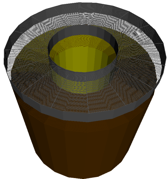
Figure 1. Left panel : Simulation and post-processing software pipeline logical schema. Right panel : Geant4 mass model of the XMM-Newton mirror module including the X-ray baffle placed at the telescope pupil.
