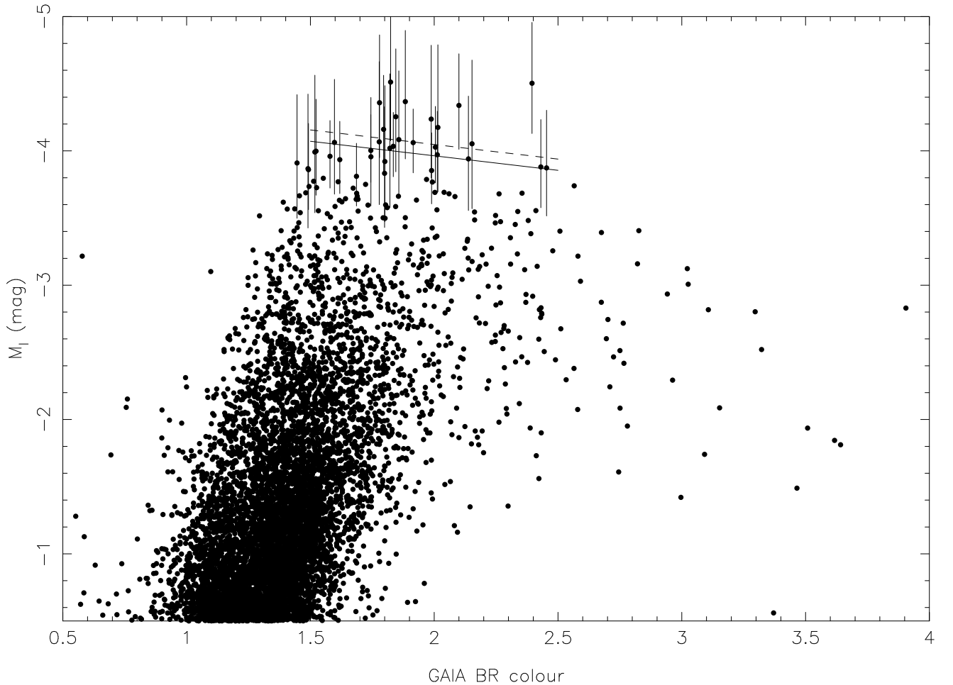
Figure 1. SkyMapper Gaia DR2 red giant branch. The axis labelled BR colour is G_{BP} - G_{RP} . Parallax uncertainties are shown for the brightest stars. A calibration of the TRGB by Rizzi et al (2007) is the solid line. A Gaia DR2 mean parallax offset of -0.028 \pm 0.006 mas was subtracted from the data from Table 1 of Arenou et al (2018), appropriate to the Sculptor galaxy, which is at the South Galactic Pole. The dashed line represents its 6 \mu\text{as} uncertainty. The query in §2.1 also brings in stars with luminosities fainter than are plotted here.
